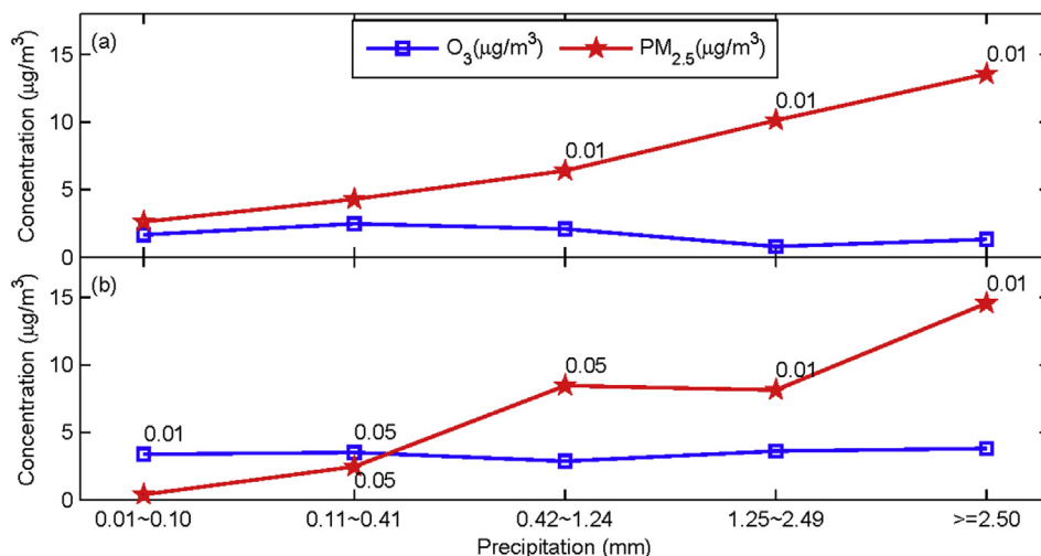
Fig. 5. Average hourly concentration differences of O_3 and PM_{2.5} between pre- and post-precipitation for each category of precipitation at the SDZ (a) and BL (b) stations (values shown in the figure denote the significance level of the differences).
