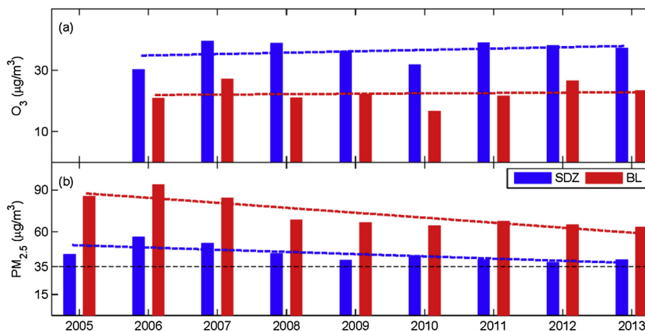
Fig. 2. Annual mean concentrations of O_3 (a) and PM_{2.5} (b) at SDZ and BL stations (Long-term trends are shown as dotted lines; the black dashed lines in (b) indicated the PM_{2.5} at the minimum safe level for the residential areas).
