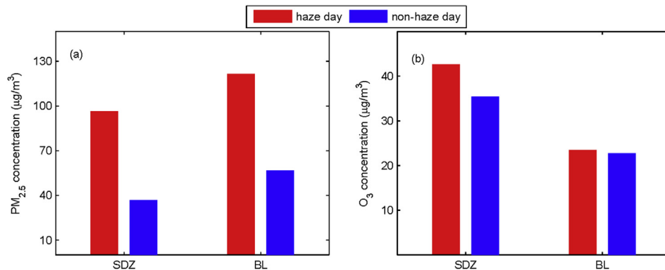
Fig. 6. Average daily concentrations of PM_{2.5} (a) and O_3 (b) on haze day and non-haze day (all of the differences were significant at the 0.01 confidence level).
