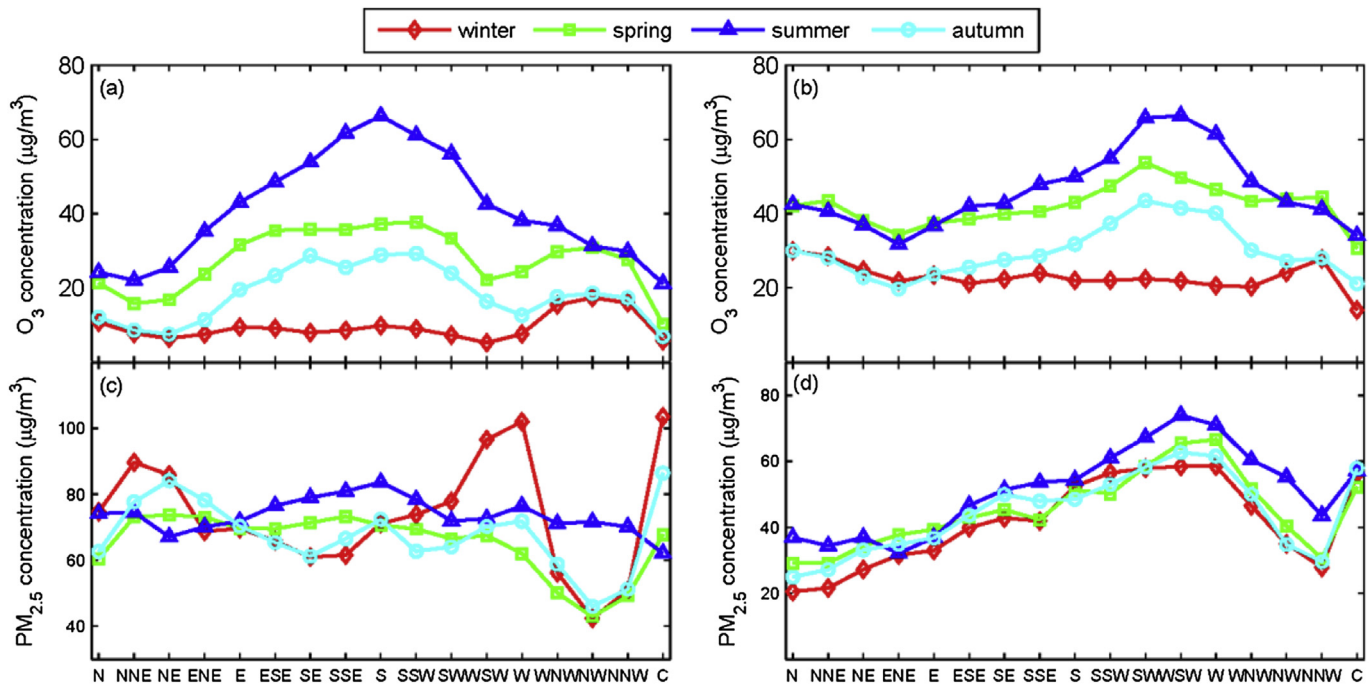
Fig. 4. Distribution of seasonal average concentrations of O_3 (a, b) and PM_{2.5} (c, d) at BL (left) and SDZ (right) stations in 16 directions (C denotes the concentrations on calm days).
