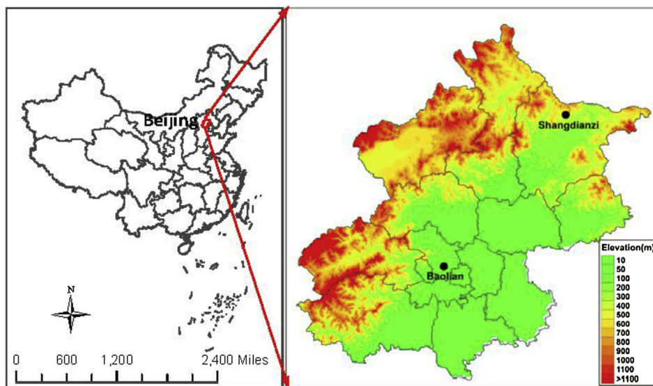
Fig. 1. Locations of the urban station of Baolian (BL) and rural station of Shangdianzi (SDZ).
