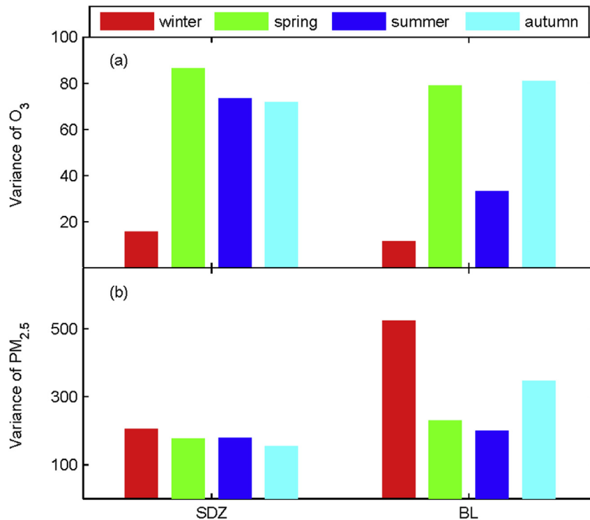
Fig. 3. Variances of the average daily variability of O 3 (a) and PM 2.5 (b) in the different seasons for the two stations.
