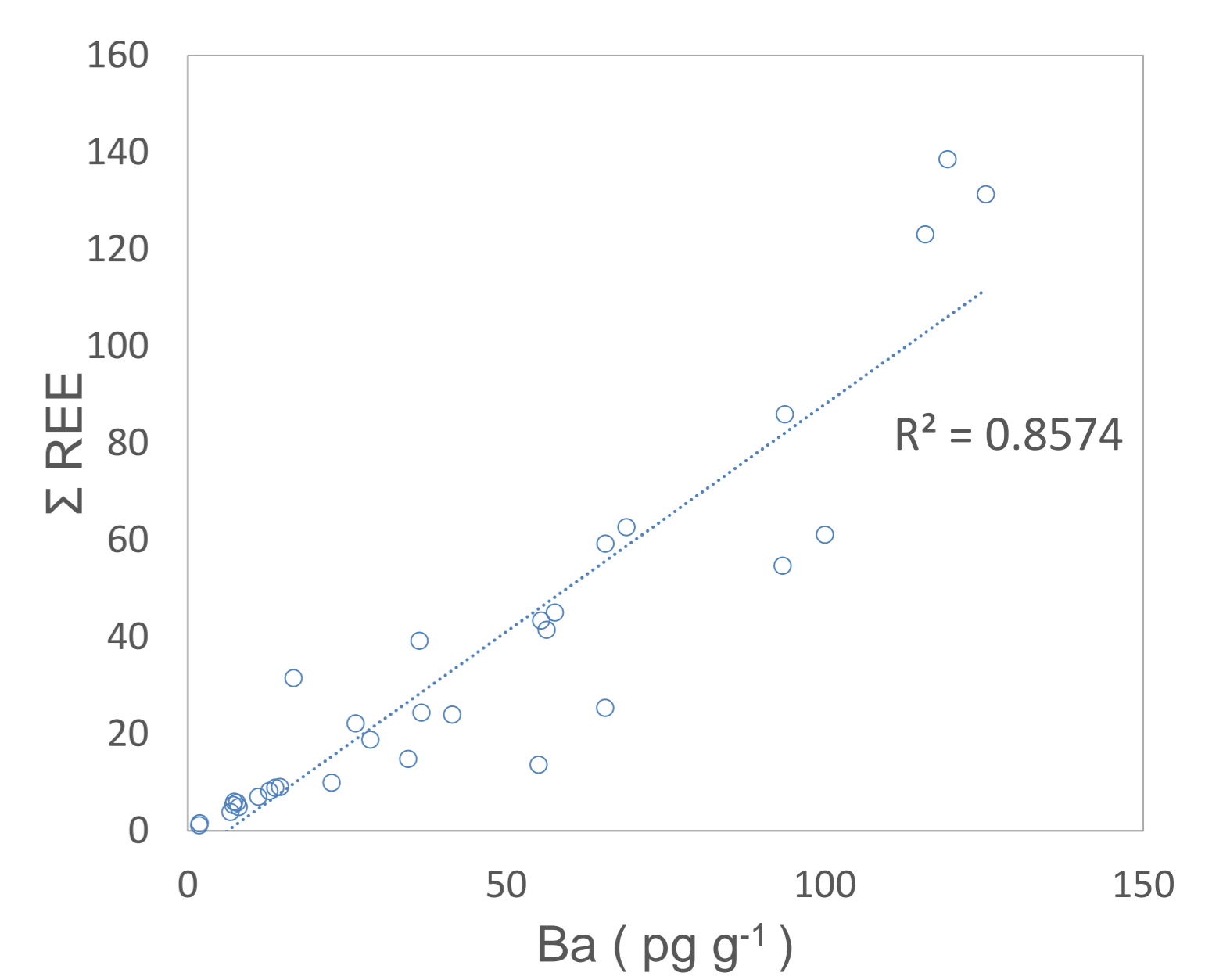
Figure 4. Correlations between sum REE and Ba concentrations
