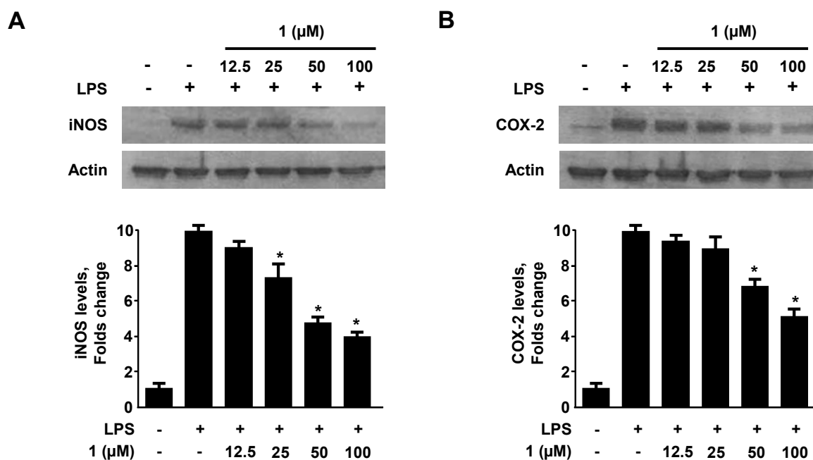
Figure 4. Effect of neoechinulin A ( 1 ) on the expression of iNOS (A) and COX-2 (B) protein. RAW264.7 macrophages were pre-treated with the indicated concentrations of neoechinulin A ( 1 ) for 3 h, and then treated with LPS (1 \mu\text{g/mL} ) for 18 h. Representative blots from three independent experiments with similar results and densitometric evaluations are shown. Data shown represent the mean values of three experiments \pm SD. * p < 0.05 as compared to the group treated with LPS alone.
