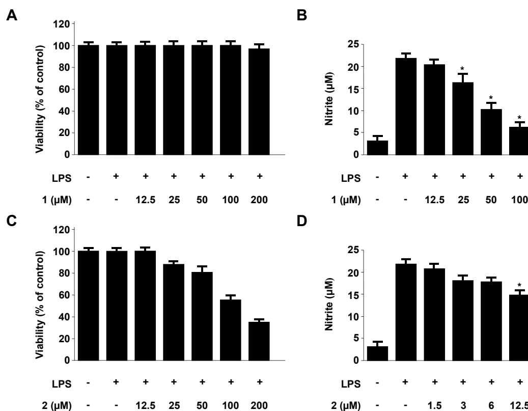
Figure 2. Effects of neoechinulins A ( 1 ) and B ( 2 ) on cell viability (A, C) and nitrite production (B, D). In the cell viability assay, RAW264.7 macrophages were incubated for 24 h with various concentrations (12.5 \mu M–200 \mu M) of neoechinulins A ( 1 ) and B ( 2 ). Cell viability was determined, as described in the materials and methods. In the nitrite production assay, RAW264.7 macrophages were pre-treated with indicated concentrations of neoechinulins A ( 1 ) and B ( 2 ) for 3 h, and then stimulated with LPS (1 \mu g/mL) for 18 h. The concentration of nitrite was determined as described in the Experimental. Data shown represent the mean values of three experiments \pm SD. * p < 0.05 as compared to the group treated with LPS alone.
