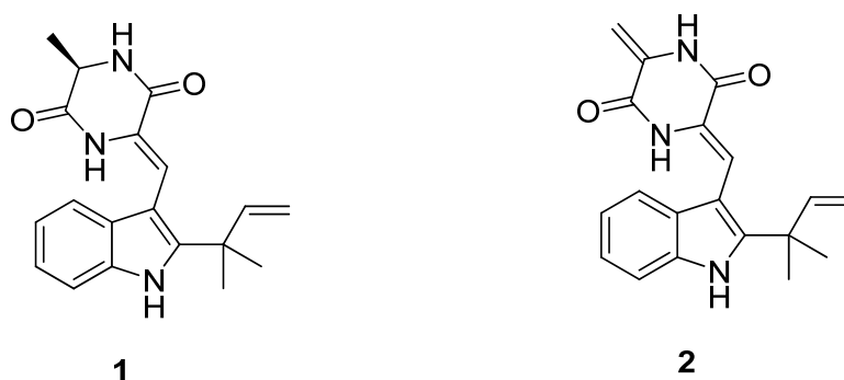
Figure 1. Chemical structures of neoechinulins A ( 1 ) and B ( 2 ).
