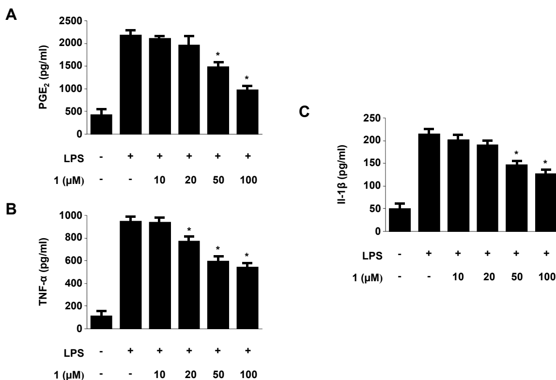
Figure 3. Effect of neoechinulin A ( 1 ) on the production of PGE 2 (A) TNF- \alpha (B), and IL-1 \beta (C). RAW264.7 macrophages were pre-treated with the indicated concentrations of neoechinulin A for 3 h, and then stimulated with LPS (1 \mu g/mL) for 18 h. The concentrations of PGE 2 (A) TNF- \alpha (B), and IL-1 \beta (C) were determined as described in the Experimental. Data shown represent the mean values of three experiments \pm SD. * p < 0.05 as compared to the group treated with LPS alone.
