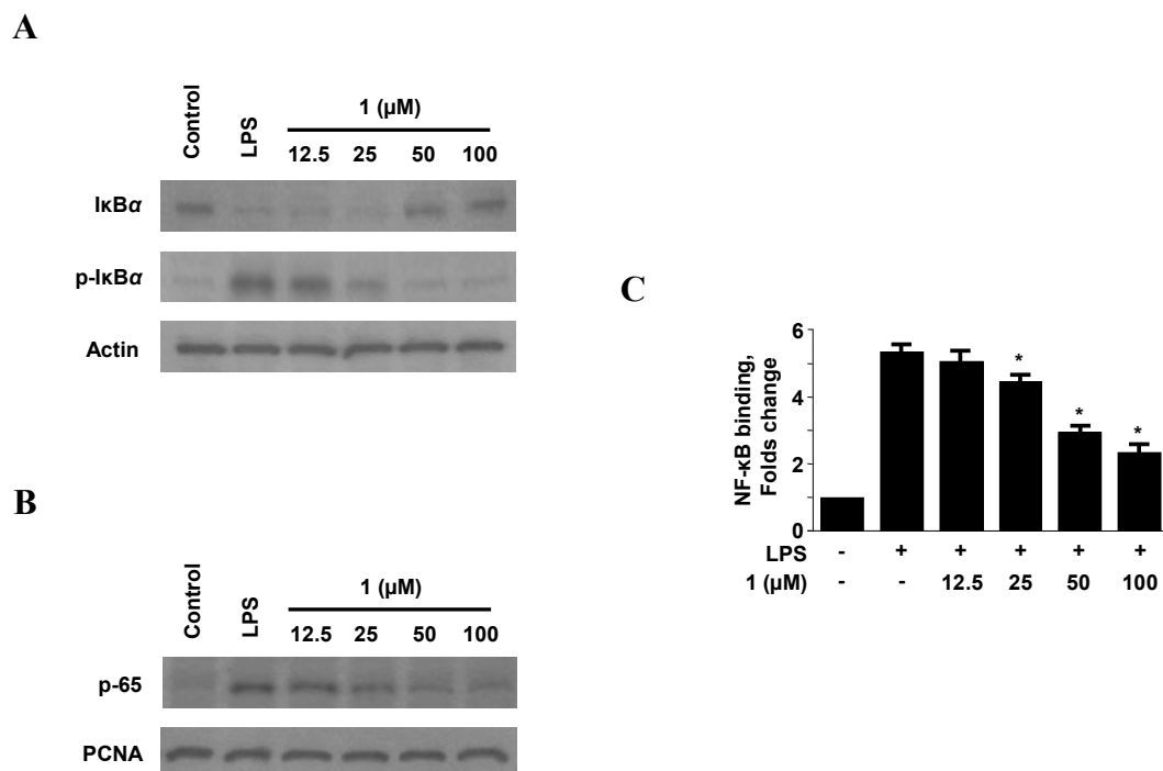
Figure 5. Effect of neoechinulin A ( 1 ) on I \kappa B- \alpha phosphorylation and degradation (A), NF- \kappa B activation (B), and NF- \kappa B DNA-binding activity (C). RAW264.7 macrophages were pre-treated with the indicated concentrations of neoechinulin A ( 1 ) for 3 h, and then stimulated with LPS (1 \mu g/mL) for 30 min. Western blot analysis was performed as described in the Experimental, and representative blots of three independent experiments are shown. A commercially available NF- \kappa B ELISA kit (Active Motif) was used to test nuclear extracts and determine the degree of NF- \kappa B binding. Data shown represent the mean values of three experiments \pm SD. * p < 0.05 as compared to the group treated with LPS alone.
