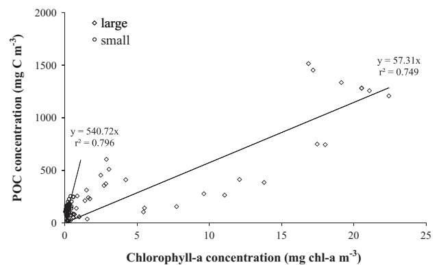
Fig. 3. Linear relationships between the particulate organic carbon (POC) and chlorophyll- a . Concentrations of small ( < 5 \mu\text{m} ) and large phytoplankton ( > 5 \mu\text{m} ).
