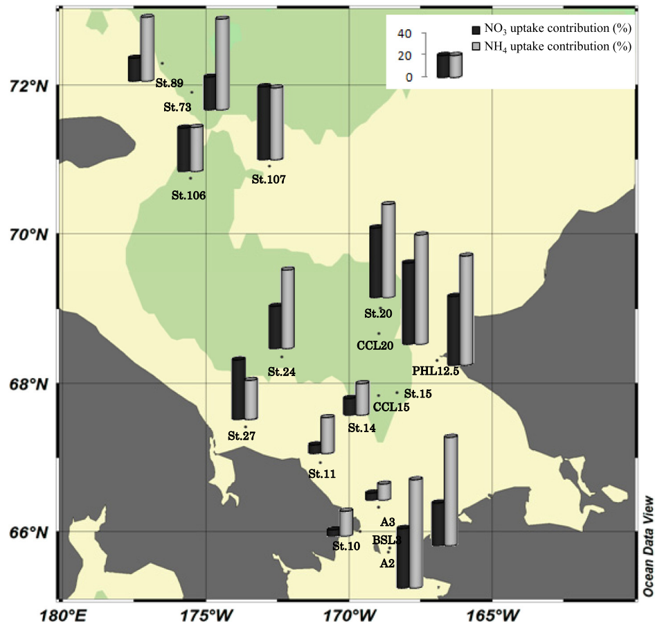
Fig. 6. Nitrate ( \text{NO}_3 ) and ammonium ( \text{NH}_4 ) uptake rate contributions of small phytoplankton in the Chukchi Sea.
