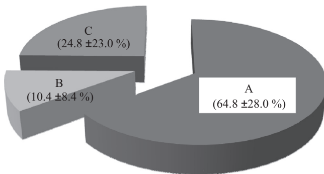
Fig. 2. Composition of different-sized cells of phytoplankton. Averages from 100, 30, and 1% light depths. (A) > 20 \mu\text{m} , (B) 5\text{--}20 \mu\text{m} , and (C) 0.7\text{--}5 \mu\text{m} .
