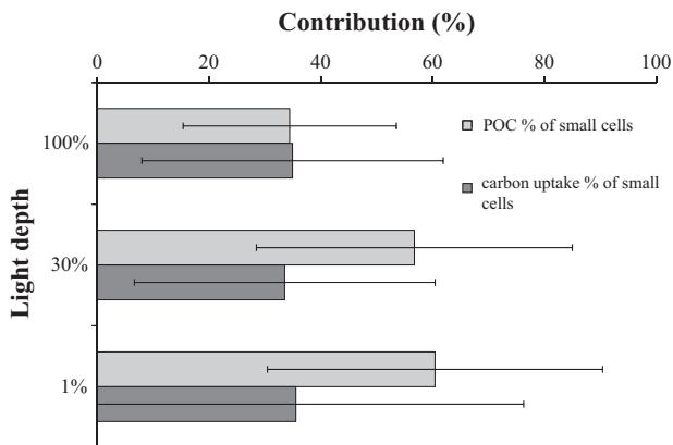
Fig. 5. Contributions of small phytoplankton at three different light depths averaged for all productivity measurement stations in the Chukchi Sea.
