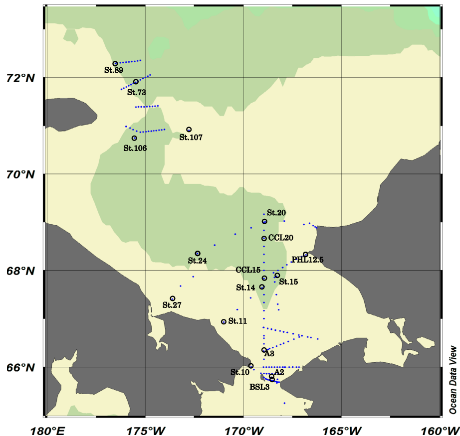
Fig. 1. Sampling locations in the Chukchi Sea, 2004. Carbon and nitrogen uptake rates were measured at the stations identified by circles. Station names with St. are those sampled during the first cruise and other stations were sampled during the second cruise.
