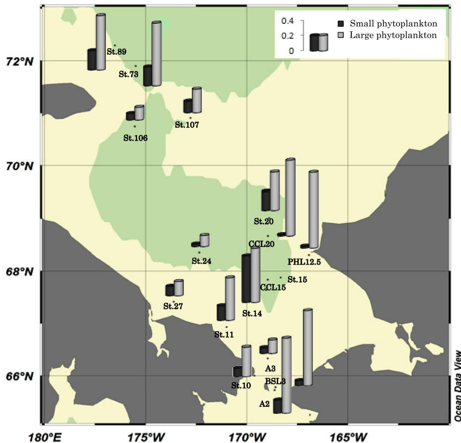
Fig. 7. Spatial distribution of the f -ratios of small and large phytoplankton in the Chukchi Sea.
