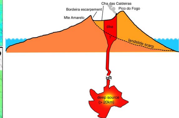
Fogo, Cape Verde - structural model
