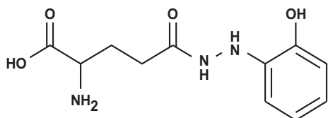
Fig. 1. Chemical structure of ramalin.
