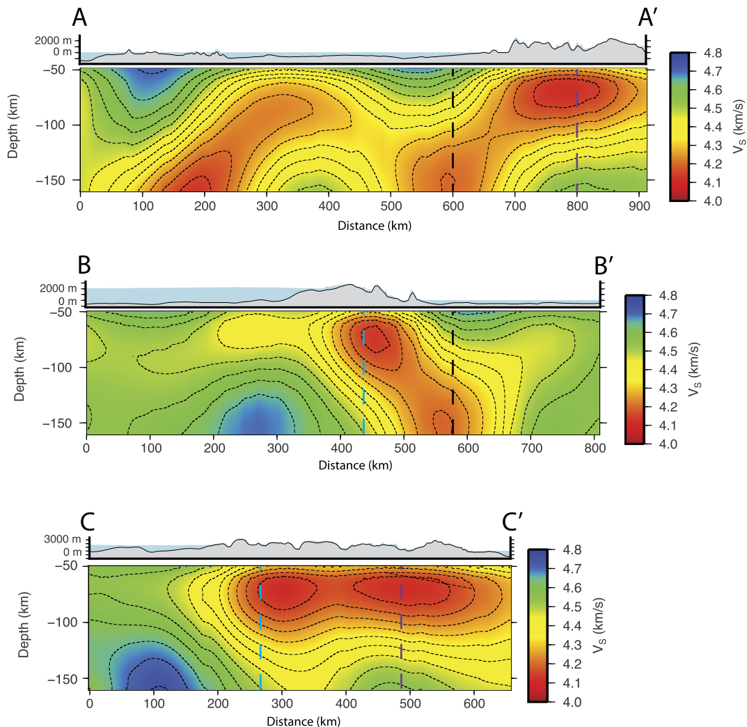
Fig. 10. Cross-sections along profiles A–A', B–B', and C–C' (locations shown on Fig. 9), with bedrock (gray) and ice (blue) topography from BEDMAP2 (Fretwell et al., 2013) shown above. Dashed lines show where the cross-sections intersect one another, matching along the black, blue, and purple dashed lines. (For interpretation of the references to color in this figure, the reader is referred to the web version of this article.)
