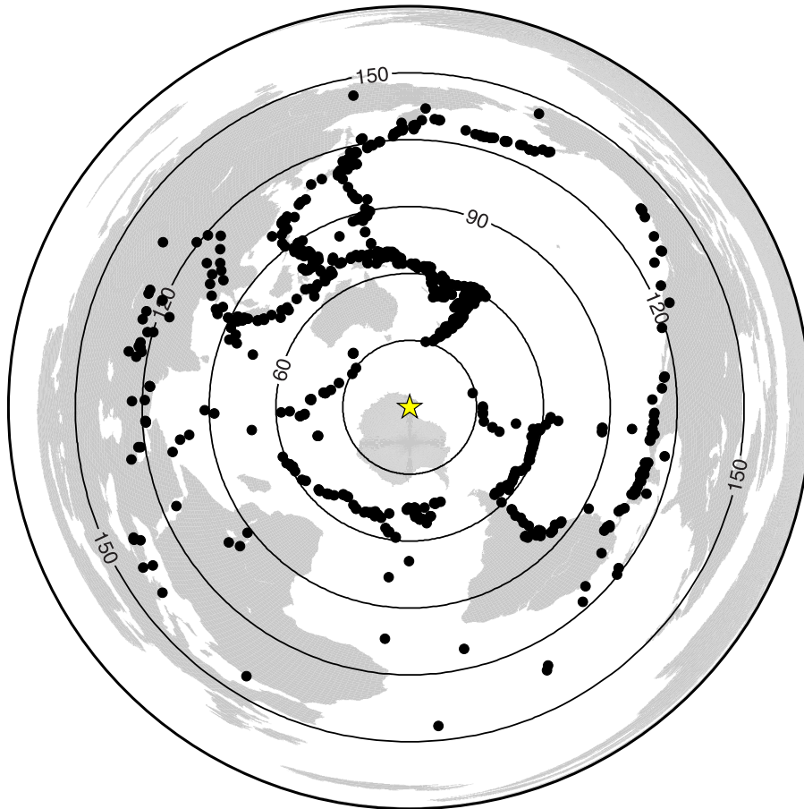
Fig. 2. Map showing the locations of all events (black dots) used in our study. The yellow star marks the center of the TAMMNET array. Concentric circles mark the epicentral distance in 30^\circ increments from the yellow star. All events lie within 30\text{--}150^\circ from the examined stations. (For interpretation of the references to color in this figure, the reader is referred to the web version of this article.)
