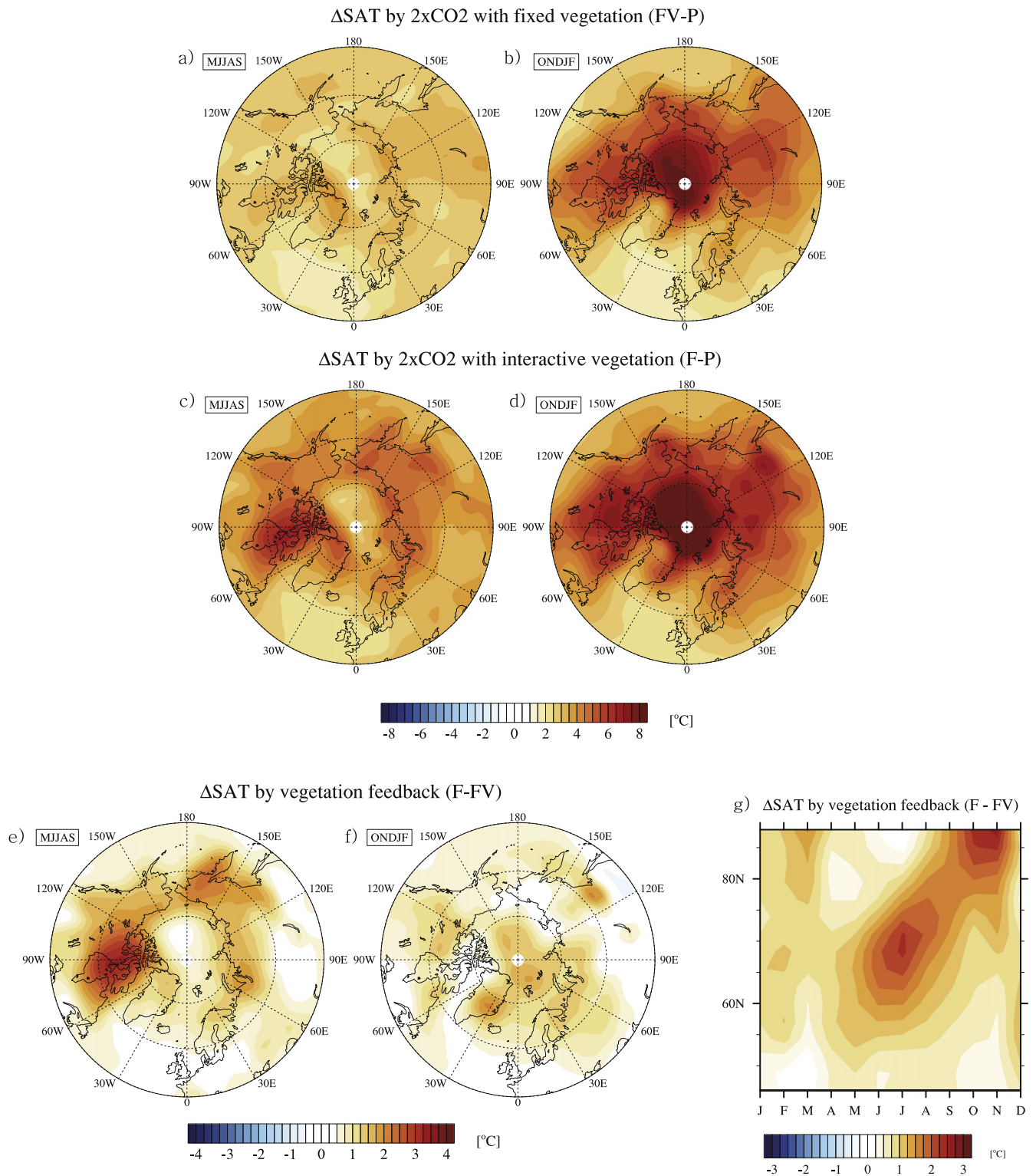
Figure 2. Surface air temperature difference between the FV and P simulation (a), (b), the F and P simulation (c), (d) and the F and FV simulation (e), (f). The zonal mean of the surface air temperature difference between the F and FV simulation (g).
