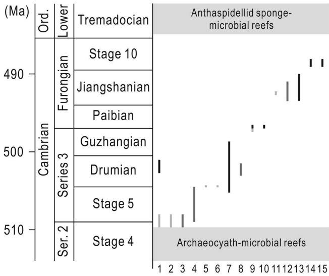
Figure 1. Occurrence of reef-building sponges and non-reef-building anthaspideiid sponges during the Cambrian Series 3–Furongian. Light gray lines: non-reef-building anthaspideiid sponges; dark gray lines: metazoan-microbial reefs not constructed by anthaspideiid sponges; black lines: reefs constructed by anthaspideiid sponges. (1) Rankenella mors , Tindall Limestone (Daly Basin) and Thornton Limestone (southern Georgina Basin), and Angulocellularia-Taninia-R. mors reef, Ranken Limestone (Undilla Sub-Basin, Georgina Basin), Australia (Kruse, 1983, 1996; Kruse and Reitner, 2014). (2) Unidentified anthaspideiid sponge, La Laza Formation (San Juan), Argentina (Beresi and Rigby, 1994). (3) Kordephyton-Jawnya gurumal-Wagima galbanyin reef, Tindall Limestone, Daly Basin, Australia (Kruse, 1996; Kruse and Reitner, 2014). (4) Orlinocyathus-Epiphyton reef, Dedebulak Formation, Kyrgyzstan (Vologdin, 1962). (5) Fieldospongia , Burgess Shale Formation, British Columbia, Canada (Rigby, 1986). (6) Capsospongia , Burgess Shale Formation, British Columbia, Canada (Rigby, 1986). (7) Epiphyton-Rankenella zhangxianensis-Cambroctoconus orientalis reef, Zhangxia Formation, Shandong Province, China (Woo, 2009; Park et al., 2011; this study). (8) Siliceous sponge- Epiphyton reef, Daegi Formation, Taebaeksan Basin, Korea (Hong et al., 2012). (9) Rankenella hamdi and R. hamdi-Girvanella reef, Mila Formation, Iran (Hamdi et al., 1995; Kruse and Zhuravlev, 2008). (10) Gallatinospongia conica -dendrolite reef, Bonanza King Formation, Nevada and California, USA (Shapiro and Rigby, 2004). (11) Gallatinospongia conica , Gallatin Formation, Wyoming, USA (Okulitch and Bell, 1955). (12) Siliceous sponge-microbial reef, Chaomidian Formation, Shandong Province, China (Lee et al., 2014a). (13) Wilbermicyathus donegani-Girvanella-Tarthinia reef, Wilberns Formation, Texas, USA (Johns et al., 2007). (14) Wilbermicyathus donegani-Girvanella-Tarthinia reef, Dotsero Formation, Colorado, USA (Johns et al., 2007). (15) Anthaspideiid sponge-microbial reef, Desert Valley Formation, Nevada, USA (Mrozek et al., 2003; Dattilo et al., 2004).
