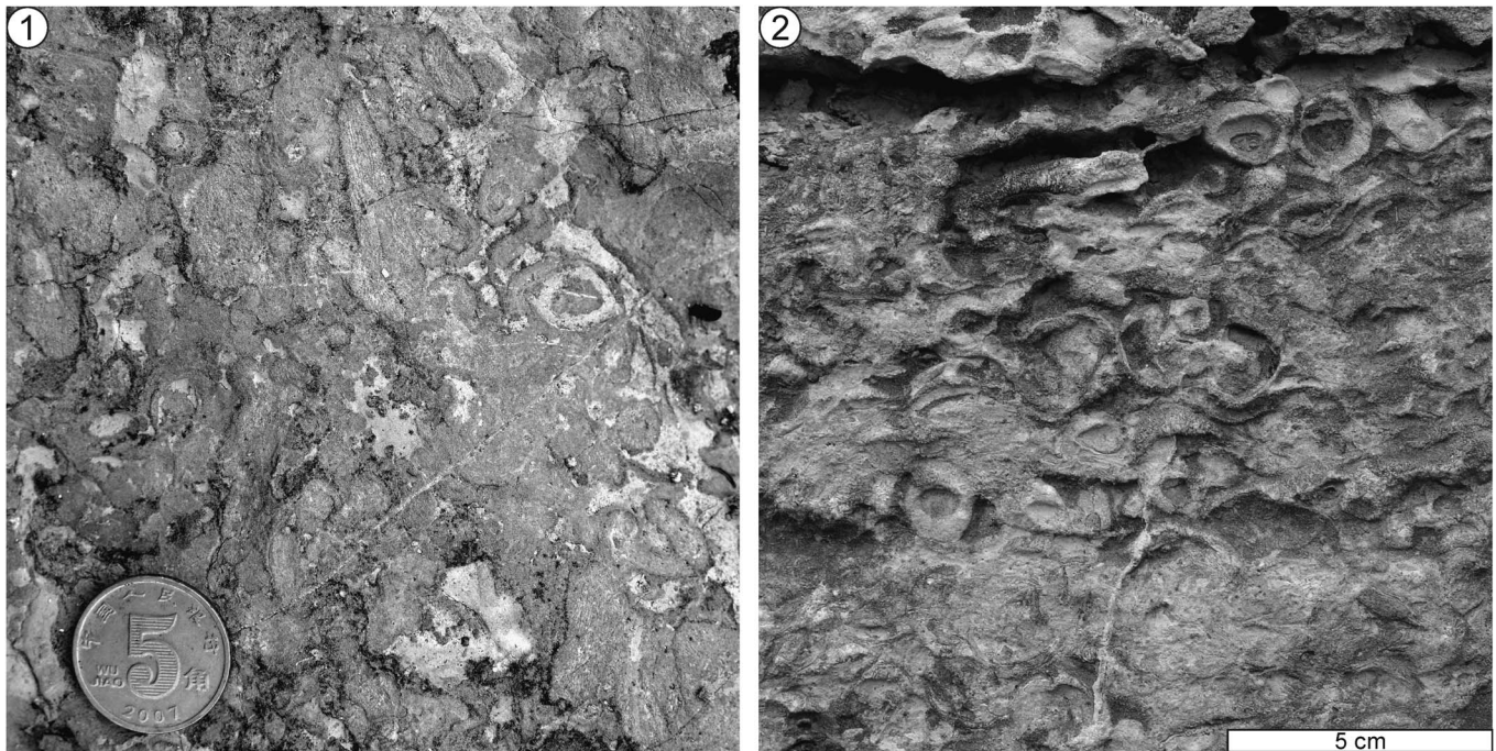
Figure 3. Outcrop photographs of Rankenella zhangxianensis in Zhangxia Formation, Beiquanzi section. For location, see Figure 2. (1) Bedding-plane view of Epiphyton-R. zhangxianensis-Cambroctoconus orientalis reef. Coin for scale is 20 mm in diameter. (2) Bedding-parallel view of R. zhangxianensis within the inter-reef grainstone.
