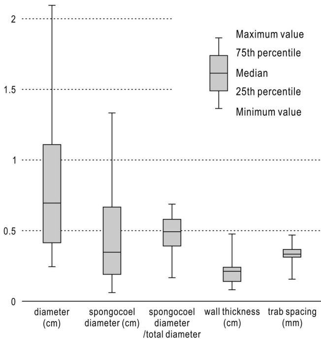
Figure 6. Box plots of measured values of some studied specimens ( n = 53 ). For raw data, see Supplementary Table 1.
