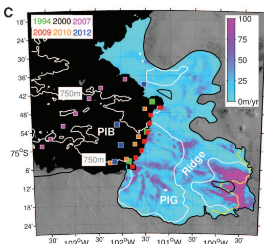
Fig. 1. Temperature maximum, seabed elevation, and selected observation locations in the Amundsen Sea.
