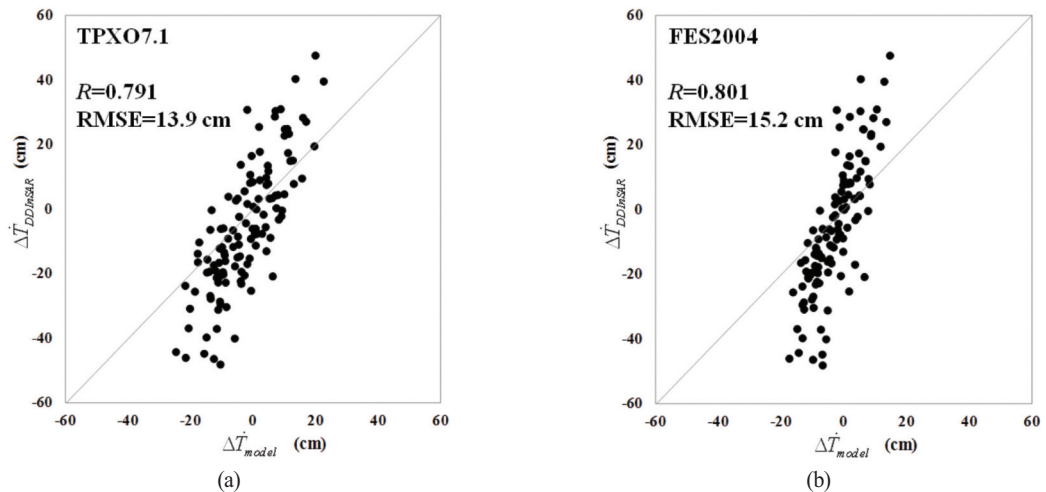
Fig. 2. Relationships between double-differential tide height for Campbell Glacier Tongue extracted from DDIInSAR images ( \Delta\dot{T}_{DDIInSAR} ) and that predicted by the tide models ( \Delta\dot{T}_{model} ) such as (a) TPXO7.1, (b) FES2004, (c) CATS2008a and (d) Ross_Inv.
