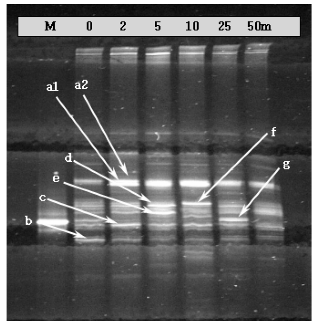
Fig. 1. DGGE band patterns of P2/P3 PCR products. Labels: M= E. coli ; 0~50 m=depth of sampling in Lake Khuvsgul; a~g=bands isolated and sequenced for identification.
