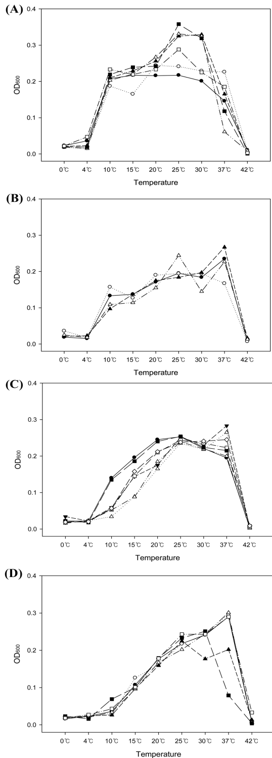
Fig. 2. Growth of 23 selected isolates in R2 broth at nine different temperatures after 48 h of cultivation. (A) Strains isolated from 0~2 m depth (Symbols: ○, 1A4; ●, 1B1; △, 1C4; ▲, 1D4; □, 1D5; ■, 1D6). (B) Strains isolated from 5 m depth (Symbols: ○, 1E1; ●, 1E2; △, 1E3; ▲, 1E6). (C) Strains isolated from 10 m depth (Symbols: ○, 2A1; ●, 2A2; △, 2A3; ▲, 2A4; □, 2A5; ■, 2A6; ◇, 2B1). (D) Strains isolated from 25~50 m depth (Symbols: ○, 2C1; ●, 2C2; △, 2C3; ▲, 2C4; □, 2C6; ■, 2F6).
