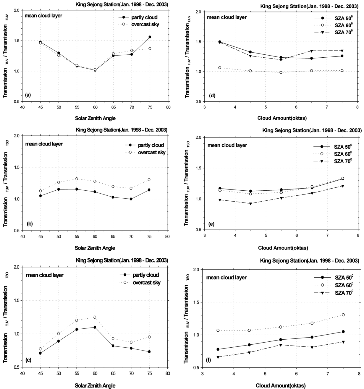
Fig. 12. Ratios between the EUV, TSO and TUV transmission; (a)(d) \frac{TUV/TUV_0}{EUV/EUV_0} , (b)(e) \frac{TUV/TUV_0}{TSO/TSO_0} and (c)(f) \frac{EUV/EUV_0}{TSO/TSO_0} as a function of SAZ and cloud amount.
