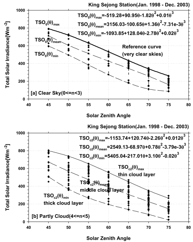
Fig. 8. Same as Fig. 6 except for total solar irradiance.
