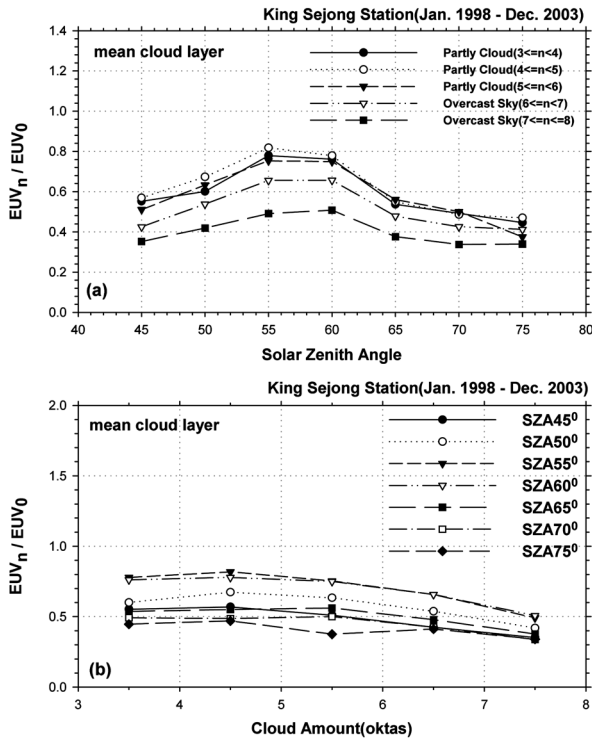
Fig. 7. EUVB transmission of mean cloud layer for maximum value under clear sky conditions as a function of (a) SZA and (b) cloud amount.
