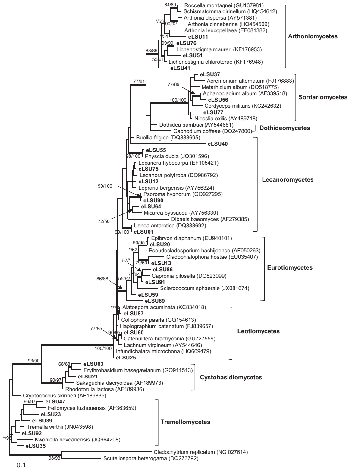
Figure 3 Maximum likelihood tree of LSU rDNA of lichen-associated fungi. Thick branches indicate those maintained in both ML and MP trees. Bootstrap values for ML and MP trees (both 1,000 replicates) are shown on corresponding branches. Tree was rooted with Scutellospora heterogama (DQ273792, Glomeromycota) and Cladochytrium replicatum (NG027614, Chytridiomycota).
