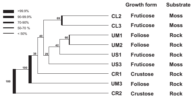
Figure 4 Jackknife sample clustering analysis of all lichen-associated fungi OTUs based on distance matrix generated by calculating pairwise FastUniFrac values. Sample clustering was based on UniFrac metric with abundance weight option on. Support for each branch was calculated by Jackknife analysis with 1,000 permutations.
