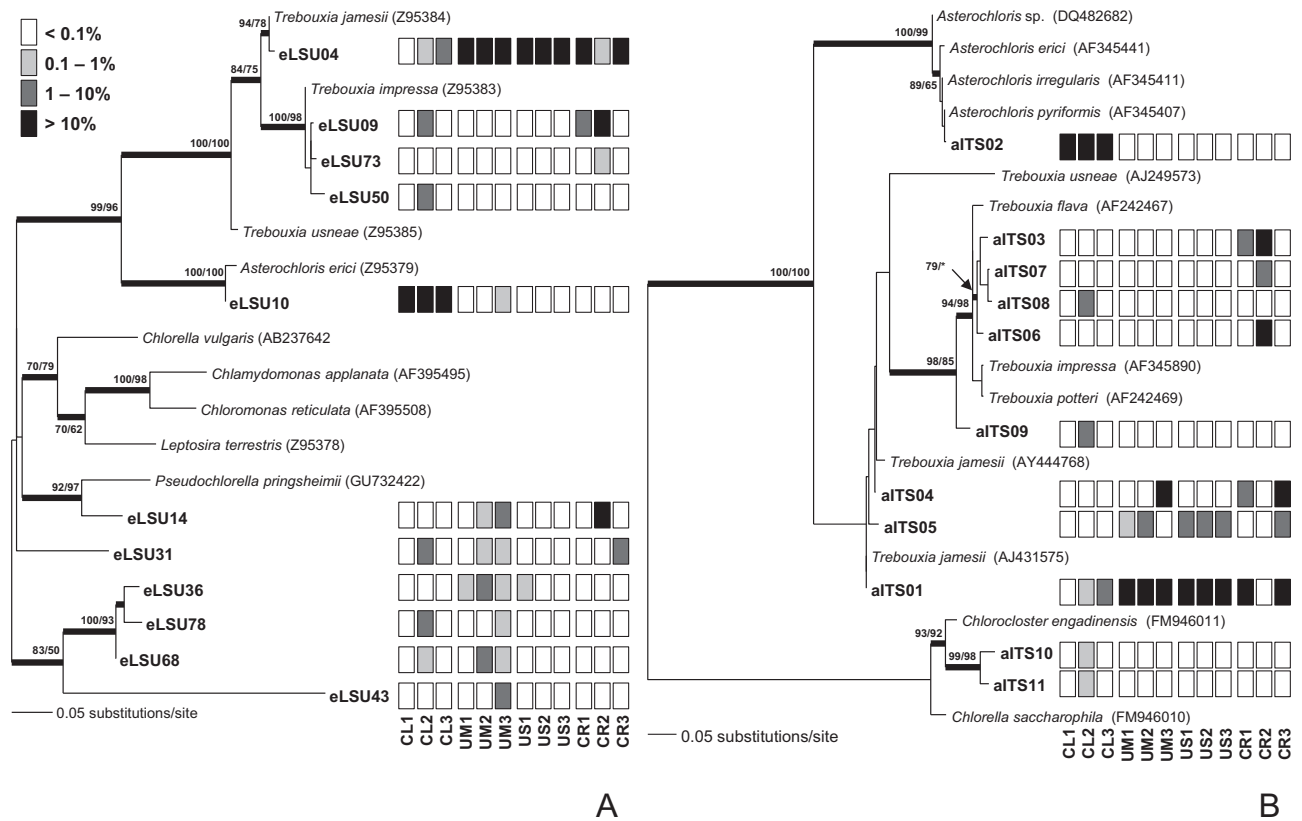
Figure 2 Maximum likelihood trees of photobiont based on sequences of A. LSU rDNA and B. algal ITS rDNA. Thick branches indicate those maintained in both ML and MP trees. Bootstrap values for ML and MP tree are shown on corresponding branches. The tree was midpoint-rooted. Intensity of shading rectangle indicates ratio (%) of the sequences.
