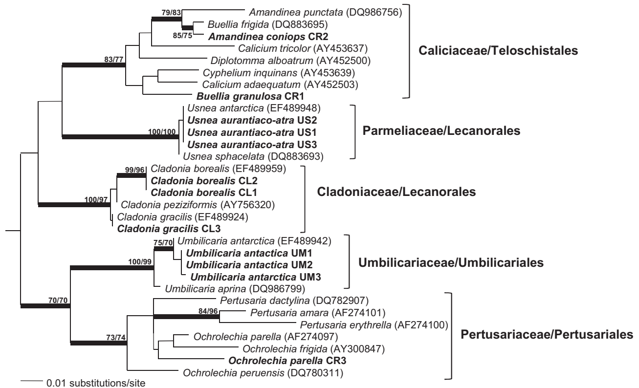
Figure 1 Maximum likelihood tree of LSU rDNA of lichenized fungi from 12 lichen samples. Thick branches indicate those maintained in both ML and MP trees. Bootstrap values for ML and MP trees (both 1,000 replicates) are shown on corresponding branches. The tree was rooted with Ascocoryne sarcoides (FJ176886, Leotiomyces).
