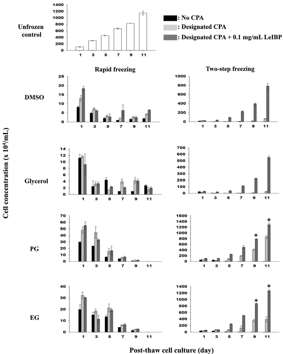
Fig. 1 Cryopreservation effect of cryoprotective agents (CPAs) on cell recovery of P. tricornutum . Cells were frozen for 2 weeks in freezing media containing different CPAs with or without 0.1 mg/ml of an antifreeze protein from the Arctic yeast Leucosporidium sp. AY30, LeIBP. Fresh cells served as unfrozen control. Post-thaw recovery was determined by neutral red staining using a hemocytometer. Error bars represent the standard deviation of three individual experiments. Asterisks indicate no significant difference between each CPA and unfrozen control ( p > 0.01 )
