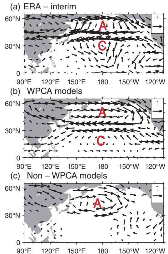
Figure 5. Regressed MAM 300-hPa wind ( \text{m s}^{-1} ) anomalies against the spring AO index for (a) the ERA-interim reanalysis, (b) the MME of the ‘WPCA’ models and (c) the MME of the ‘non-WPCA’ models. The ‘A’ and ‘C’ denote the centres of the anticyclonic and cyclonic anomalies, respectively. Only the wind vectors that exceed 0.2 \text{ m s}^{-1} are plotted.
