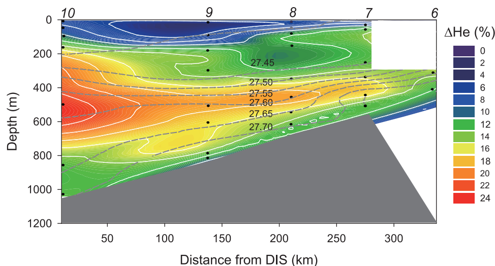
Figure 6. Distributions of \Delta\text{He} within the water column of the DT (Sts. 6–10) in 2011. The black dots indicate the sampling depth, and the grey dotted lines indicate the isopycnal lines of \sigma_\theta of 27.4–27.7. The shelf break is located near St. 7 (~280 km from the DIS, St. 10).
