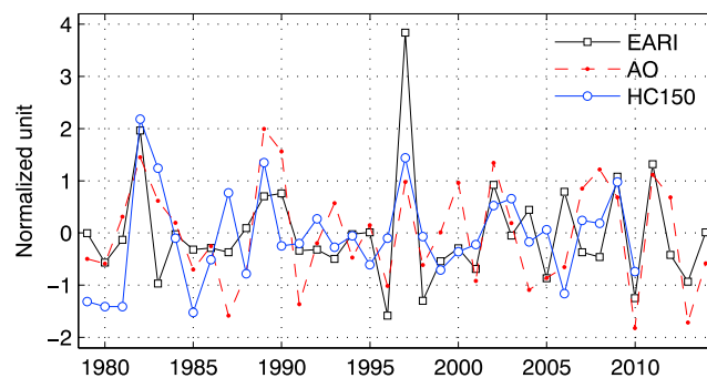
Figure 3. Time series of the JFM AO index, October East African rainfall index (EARI), and the ocean heat content in the uppermost 150 m (HC150) averaged over 40^{\circ} – 60^{\circ} E and 5^{\circ} – 10^{\circ} S. All time series are normalized with respect to the whole data period to facilitate comparison.
