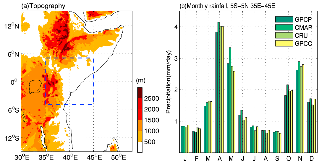
Figure 1. (a) Topography of East Africa, (b) long-term means of the monthly precipitation over the region of 5°S–5°N and 35°E–45°E with respect to 1981–2010. Target region is shown as the box in Figure 1a).
