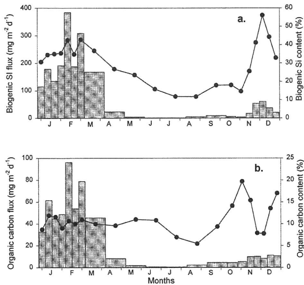
Fig. 5. Temporal evolution of a. biogenic Si fluxes and contents, and b. organic carbon fluxes and contents in eastern Bransfield Strait. Vertical bars indicate fluxes and closed circles contents.
