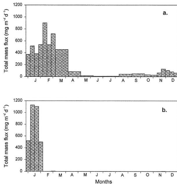
Fig. 4. Temporal evolution of mass fluxes at a. KAST 1 from 27 December 1999–27 December 2000, and b. KAST 2 from 27 December 1999–24 December 2000.
