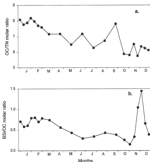
Fig. 6. Temporal evolution of a. OC/TN molar ratio, and b. BSi/OC molar ratio in eastern Bransfield Strait.
