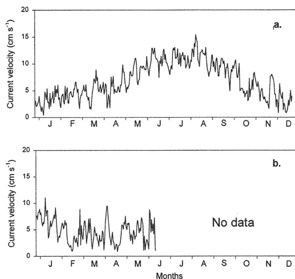
Fig. 3. Daily averaged current velocity at a. KAST 1, and b. KAST 2. At KAST 2, current data were not available after mid-June due to malfunctioning current meter.
