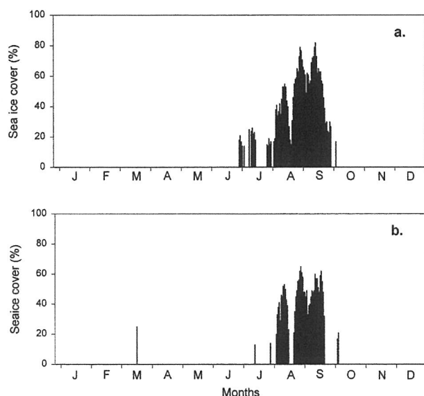
Fig. 2. Percent sea ice cover at a. KAST 1, and b. KAST 2 derived from daily DMSP F13 Special Sensor Microwave/Imager (SSM/I).
