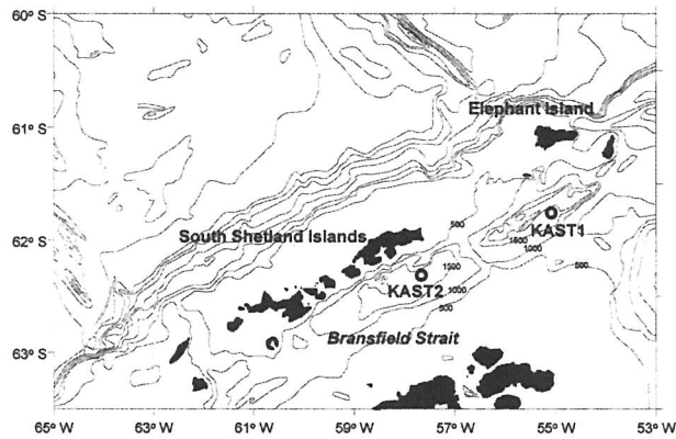
Fig. 1. Location of the sediment trap mooring sites in Bransfield Strait. The mooring sites are marked by open circles.
