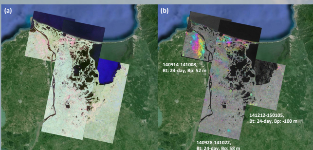
Figure 3 (a) Pauli decomposition of RADARSAT-2 SAR image as color composite image: HH+VV (red), HH+VH (blue), and VH (green). (b) Interferograms over three tracks: low coherence was found despite of small temporal and perpendicular baselines.
