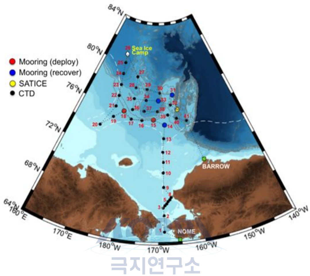
Fig. 1. Study area and sediment trap mooring stations (st. 15 and 18, red circle)
