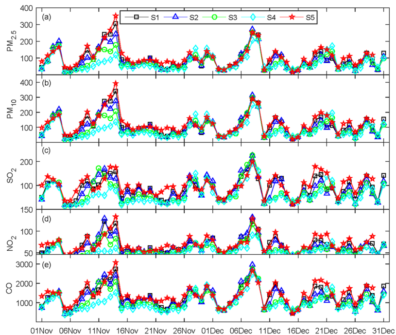
Figure 5. The daily concentrations of PM 2.5 (a), PM 10 (b), SO 2 (c), NO 2 (d) and CO (e) in downtown Beijing during November-December 2015 derived from the simulations using different scenarios in \mu\text{g}/\text{m}^3 .
