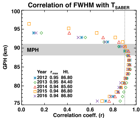
Figure 3. The height profile of correlation coefficient of the FWHM and SABER temperatures in 2012–2016. The height information of the maximum correlation coefficient and its value in each year are also summarized. The dotted vertical line indicates a correlation coefficient of 0.9, and the gray shaded box denotes the height range of the MPH variation during the observation period.
