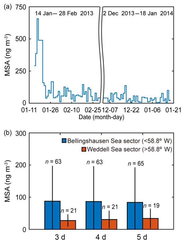
Figure 4. (a) Daily concentration of MSA collected at the sampling site during the summer periods in 2013 and 2014 (explicitly, from 14 January to 28 February in 2013 and from 2 December 2013 to 18 January 2014). (b) The mean MSA concentration that potentially originated from the Bellingshausen Sea sector (< 58.8° W) and the Weddell Sea sector (> 58.8° W) estimated by applying 3, 4 and 5 d air mass back trajectories during the austral summer periods in 2013 and 2014. The error bars indicate 1 standard deviation ( 1\sigma ) from the mean values.
