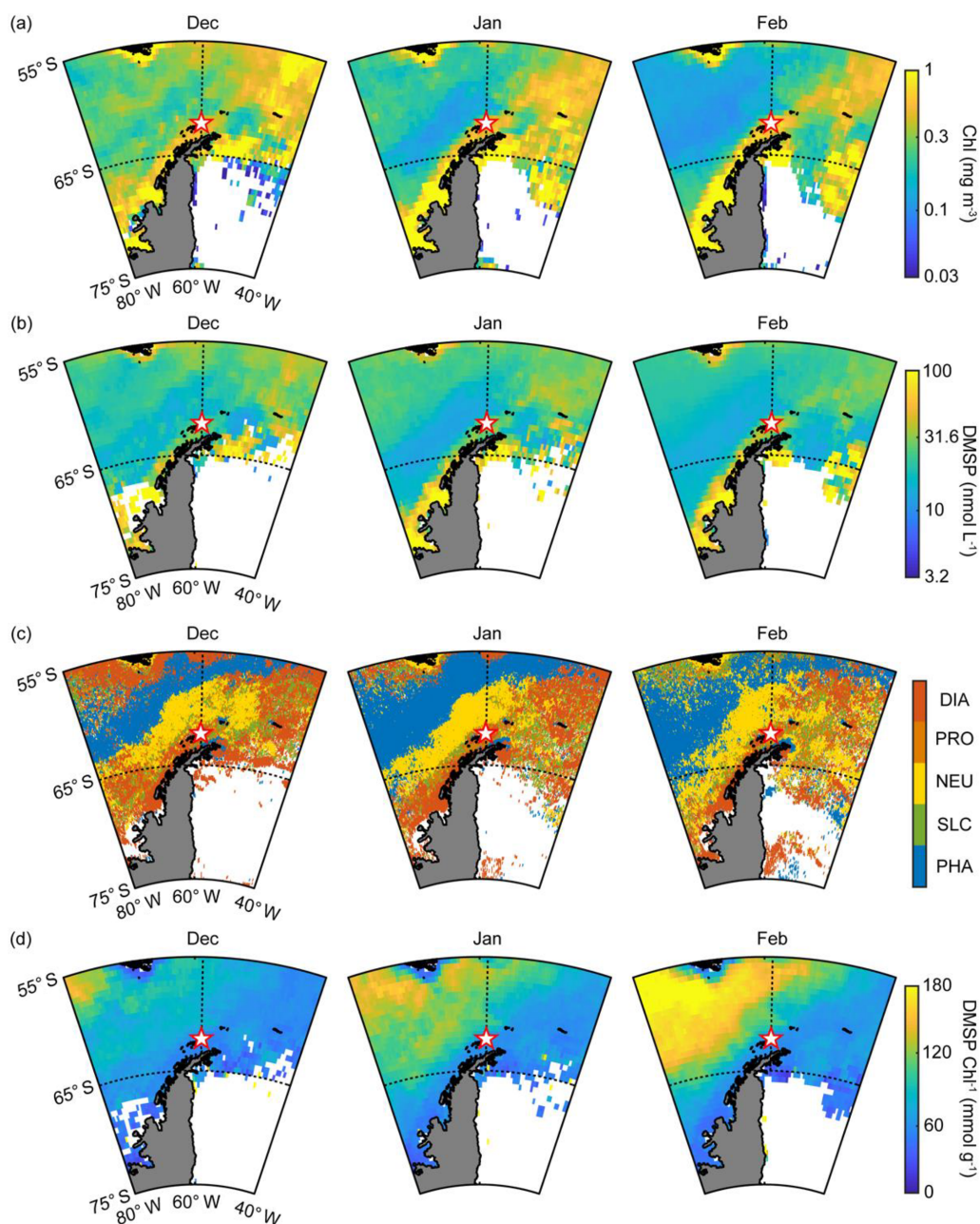
Figure 3. (a) Monthly mean chlorophyll concentration during the months of December, January and February in 2009–2016; (b) monthly mean DMSP concentration during the months of December, January and February in 2009–2016; (c) phytoplankton taxonomic composition including diatoms (DIA), Prochlorococcus (PRO), nanoeucaryotes (NEU), Synechococcus (SLC) and Phaeocystis (PHA) estimated using the PHYSAT method with the climatology map obtained from the SeaWiFS archive; and (d) monthly mean DMSP-to-chlorophyll ratio during the months of December, January and February in 2009–2016.
