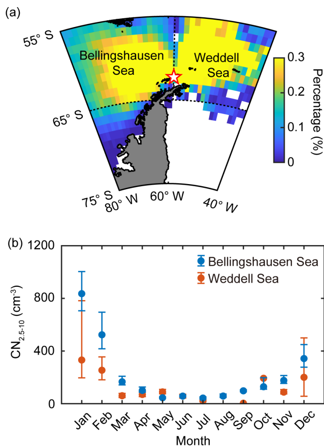
Figure 2. (a) Back trajectories of the air masses arriving at King Sejong Station (62.2° S, 58.8° W; star symbol), Antarctic Peninsula. The colors indicate the percentage (%) of the air mass located at that spot during the 2 d prior to arriving at the observation site. Note that the air mass back trajectories that did not have > 90 % retention in the two selected ocean domains (i.e., Bellingshausen and Weddell seas) were excluded. (b) Seasonal variation of nanoparticles (2.5–10 nm in diameter, CN 2.5–10 ) observed at King Sejong Station between March 2009 and December 2016. Blue and red symbols indicate the number concentration of nanoparticles that originated from the Bellingshausen and Weddell seas, respectively. The error bars indicate the 95 % confidence interval estimated by bootstrap method from the monthly CN 2.5–10 data.
