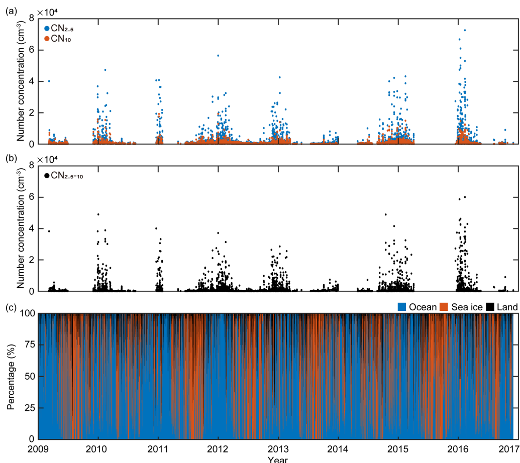
Figure 1. (a) Hourly variations in the number concentration of particles > 2.5 nm in diameter ( CN_{2.5} , blue symbols) and the number concentration of particles > 10 nm in diameter ( CN_{10} , red symbols), (b) hourly variations in the number concentration of nanoparticles (ranging from 2.5 to 10 nm in diameter) calculated using the differences between CN_{2.5} and CN_{10} , and (c) hourly variations in the retention time of 2 d air mass back trajectories over the three domains including ocean (blue), sea-ice (red), and land (black) domains from March 2009 to November 2016.
