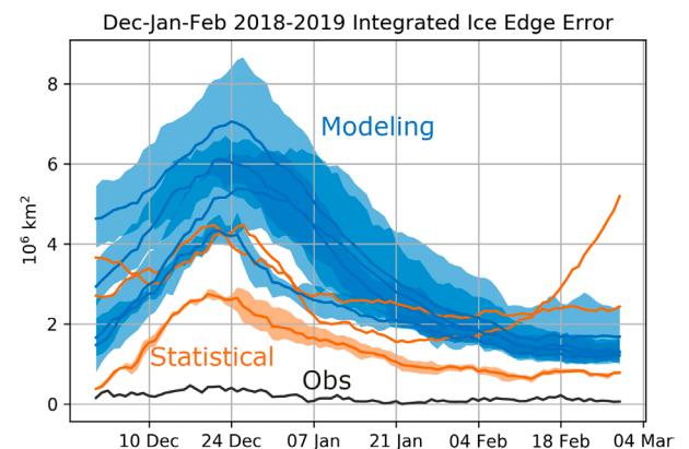
Fig. 12. Integrated ice edge error (IIEE; Goessling et al. 2016), a measure of spatial agreement of forecasted and observed sea ice concentration, for dynamical model (blue) and statistical (orange) contributions participating in the austral summer 2018/19 SIPN South coordinated forecast. The common reference verification product is NSIDC-0081 ( https://nsidc.org/data/nsidc-0081 ). Low values indicate high skill, the shadings (when available) indicate the ensemble range for a given forecasting system. The black line is the IIEE for an alternative observation product and is meant to represent uncertainty in the verification product itself.
