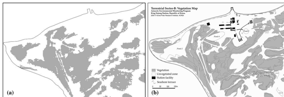
Fig 2. Vegetation coverage map by (a) SMA estimation and (b) modified vegetation map by Kim et al. (2007) around King Sejong Station, where, gray color indicates vegetated area
