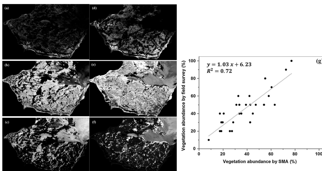
Fig 1. (a)–(f) Estimated abundance image acquired from KOMPSAT-2 and QuickBird as a linear scale 0 – 1. (a, d: Vegetation, b, e: bare surface, c, f: snow) / (g) Relationship of vegetation abundance between field survey and SMA estimation
