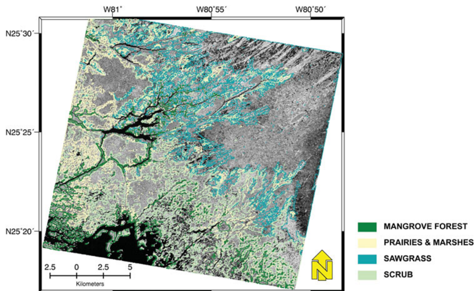
FIG. 5. RADARSAT-2 amplitude image with polygons of vegetation class that is used for coherence calculation.
