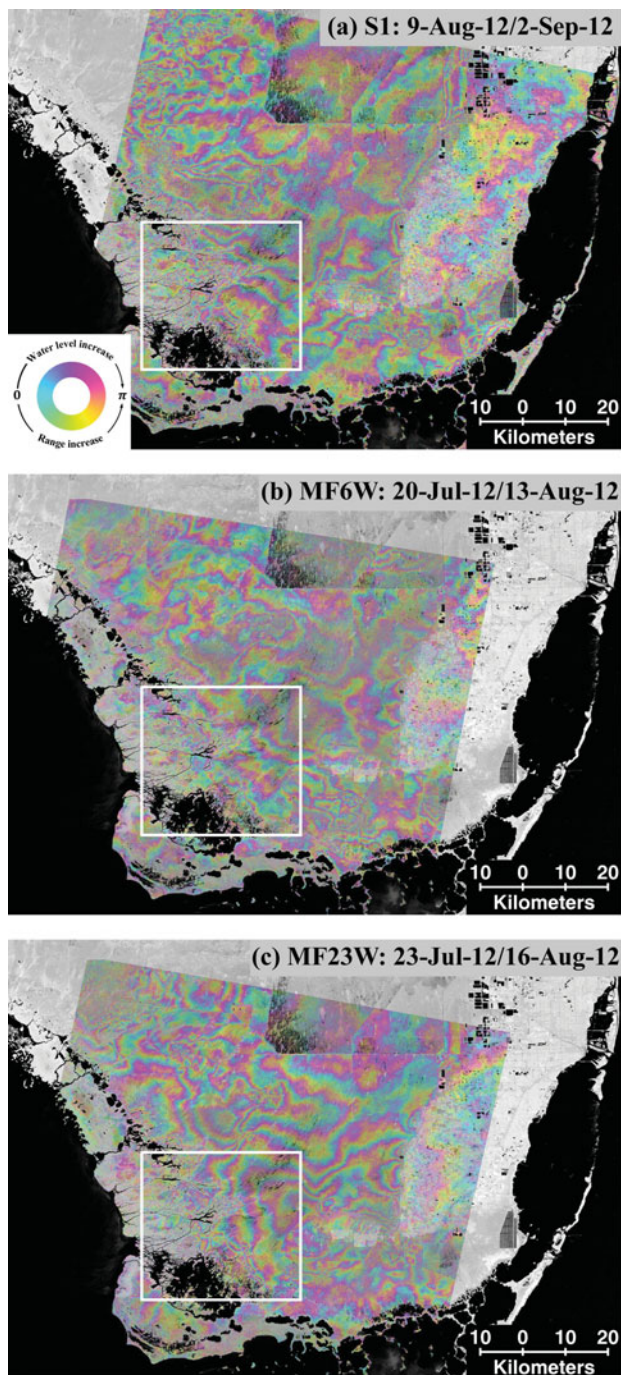
FIG. 2. Three representative interferograms covering most of Everglades National Park. The interferograms are wrapped and unfiltered to demonstrate the actual phase resolution detected by each acquisition mode. All interferograms show high coherence levels and variable fringe patterns in the freshwater wetlands located in the upper right side of the images. They also show low coherence over the mangrove forest area, on the left side of the interferograms. The white frames mark the location of the zoomed-in area presented in Figure 3.
