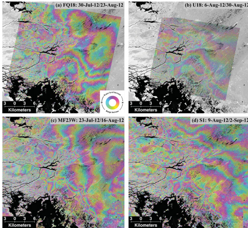
FIG. 3. Zoomed-in interferograms of the Tarpon Bay area, which is a transition zone between freshwater wetlands to the northeast and mangrove forests in the southwest. The Tarpon Bay and other tidal channels in the area are homes for the easternmost mangrove communities in the western Everglades. The interferograms show high coherence with low fringe gradients in the northeast area, which reflect water-level changes in the steady flowing freshwater wetlands. They also show low coherence over the mangrove forests in the southwest sections. Some of the interferograms also show high gradient fringes around the Tarpon Bay, reflecting water-level changes induced by tidal flow.
