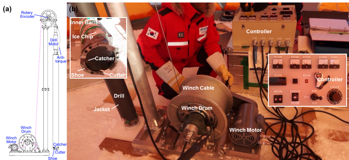
Fig. 2. (a) The design of the drilling system. Only one of three anti-torque blades is depicted. (b) The picture of the drill installed in the drilling tent. The insets show the inner barrel containing an ice core (left) and the controller (right).
