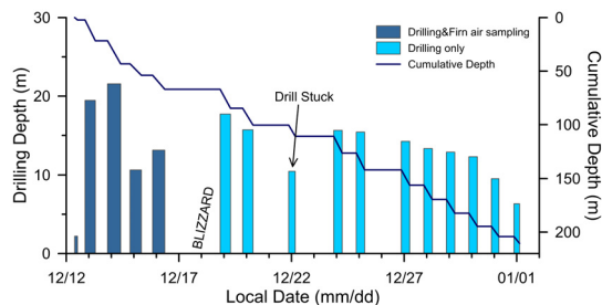
Fig. 4. The drilled depth per day (bar) and the cumulative drilled depth (line). The firm air sampling and the ice drilling were performed alternately during 12-17 December 2014.
