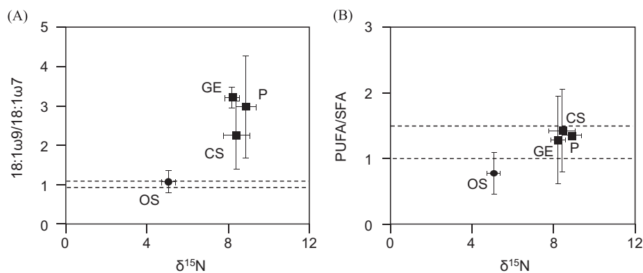
Fig. 3. Euphausia superba (●) and Euphausia crystallorophias (■). Interspecies and spatial variation of (A) 18:1 \omega 9/18:1 \omega 7 and (B) PUFA/SFA with \delta^{15}\text{N} values. The two dotted lines indicate the standard range (minimum to maximum) of a carnivore (Cripps and Atkinson, 2000; Falk-Petersen et al., 2000; Virtue et al., 2000). OS: open sea; CS: continental shelf; P: middle of polynya; GE: polynya near glacial edge.
