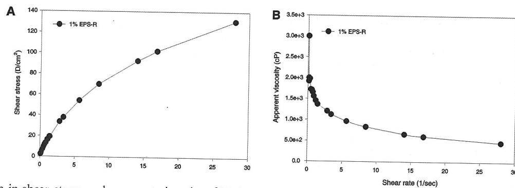
Fig. 8. Variation in shear stress and apparent viscosity of EPS-R 1.0% (w/v) fluid (A, Relationship between shear stress and shear rate of EPS-R 1.0% solution; B, Relationship between apparent viscosity and shear rate of EPS-R 1.0% solution).
