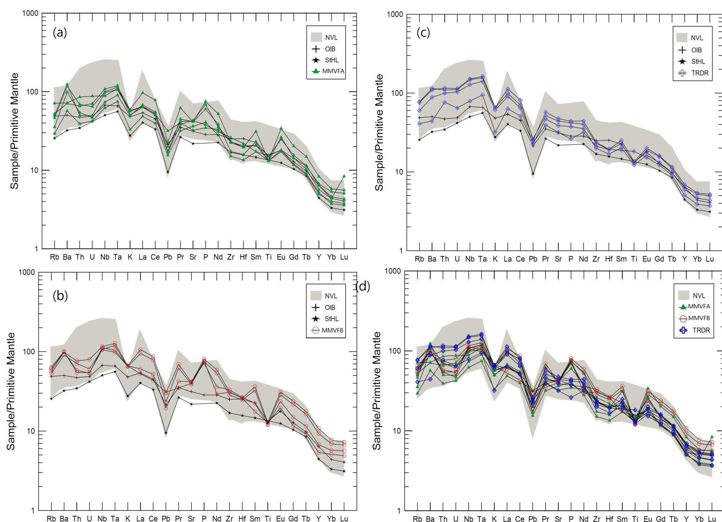
Fig. 4. Trace element patterns normalized to primitive mantle for the MMVF basalts and Terror Rift submarine lavas. Patterns of the studied samples and average OIB are compared with those of McMurdo Volcanic Group basalts from NVL and St. Helena HIMU-OIB. Data sources for comparison are: average OIB, McDonough and Sun (1995); NVL, Nardini et al. (2009); St. Helena, PETDB database ( http://www.petdb.org/index.jsp ).
