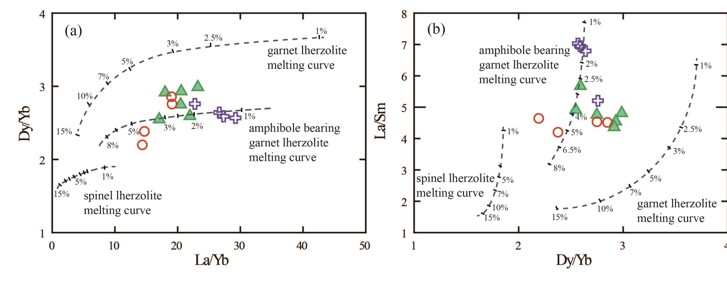
Fig. 5. Calculated partial melting curves assuming non-modal batch melting of spinel, garnet and amphibole-bearing garnet lherzolite. Phase proportions in solid and melt modes for a hypothetical spinel lherzolite used for model calculations are ol 0.578 + opx 0.27 + cpx 0.119 + sp 0.033 and ol 0.1 + opx 0.27 + cpx 0.5 + sp 0.13 , and for a hypothetical garnet lherzolite ol 0.598 + opx 0.211 + cpx 0.115 + gt 0.115 and ol 0.05 + opx 0.20 + cpx 0.30 + gt 0.45 , respectively. Phase proportions in solid and melt modes for a hypothetical amphibole-bearing garnet lherzolite are ol 0.514 + opx 0.213 + cpx 0.123 + gt 0.075 + amp 0.075 and ol 0.05 + opx 0.18 + cpx 0.205 + gt 0.25 + amp 0.315 , respectively. Modeling used the REE distribution coefficients of McKenzie & O'Nions (1991) and Chazot et al. (1996). The spinel and garnet lherzolite mantle compositions are from Tang et al. (2006). The amphibole-bearing garnet lherzolite composition is from McCoy-West et al. (2010). Abbreviations: ol, olivine; opx, orthopyroxene; cpx, clinopyroxene; sp, spinel; gt, garnet; amp, amphibole.
