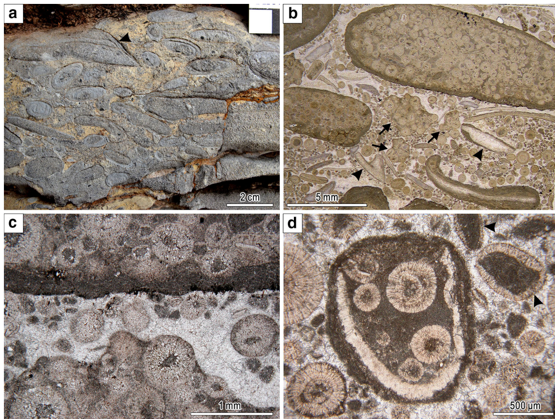
Fig. 5 Thin-cortex oncoids. a Outcrop photo, showing large nuclei and thin cortex of the oncoids. Arrow indicates upward growth of cortices on the upper surface of the nucleus. b Possibly reworked ooid aggregates as nuclei that are coated by thin cortices. Note a micro-oncoid ( right arrow head ), a cortoid ( left arrow head ), and several
