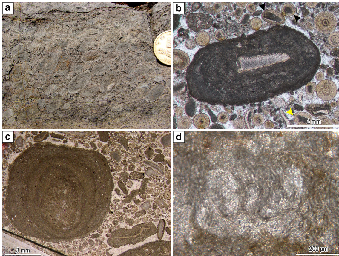
Fig. 7 Clotted-cortex oncoids. a Outcrop photo of oncoids made of thin bioclastic nuclei and cortices without distinct laminae. Coin for scale is 20.5 mm in diameter. b An ellipsoidal oncoid with a nucleus of calcareous algae and a clotted (only crudely laminated) cortex in an oolitic grainstone which contains many “ Nuia ” ooids (arrows). c An
