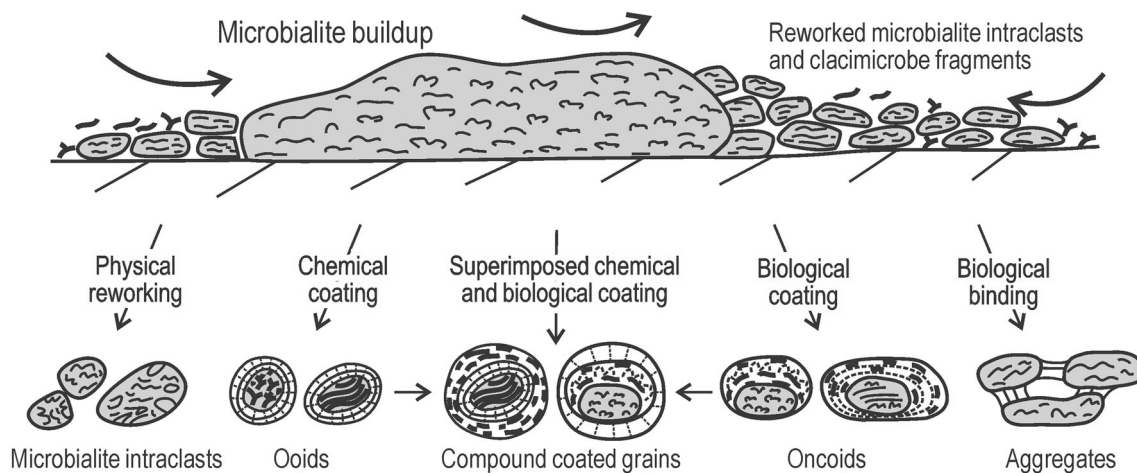
Fig. 11 Schematic model (not in scale) of microbial-related carbonate grains. Reworking of previously deposited microbialite buildups leads to formation of microbialite intraclasts and abundant calcimicrobe fragments. Some of microbialite intraclasts may resemble oncoids due to the presence of abundant calcimicrobes in both (cf. Liu and Zhang 2012). On the other hand, both the microbialite intraclasts
