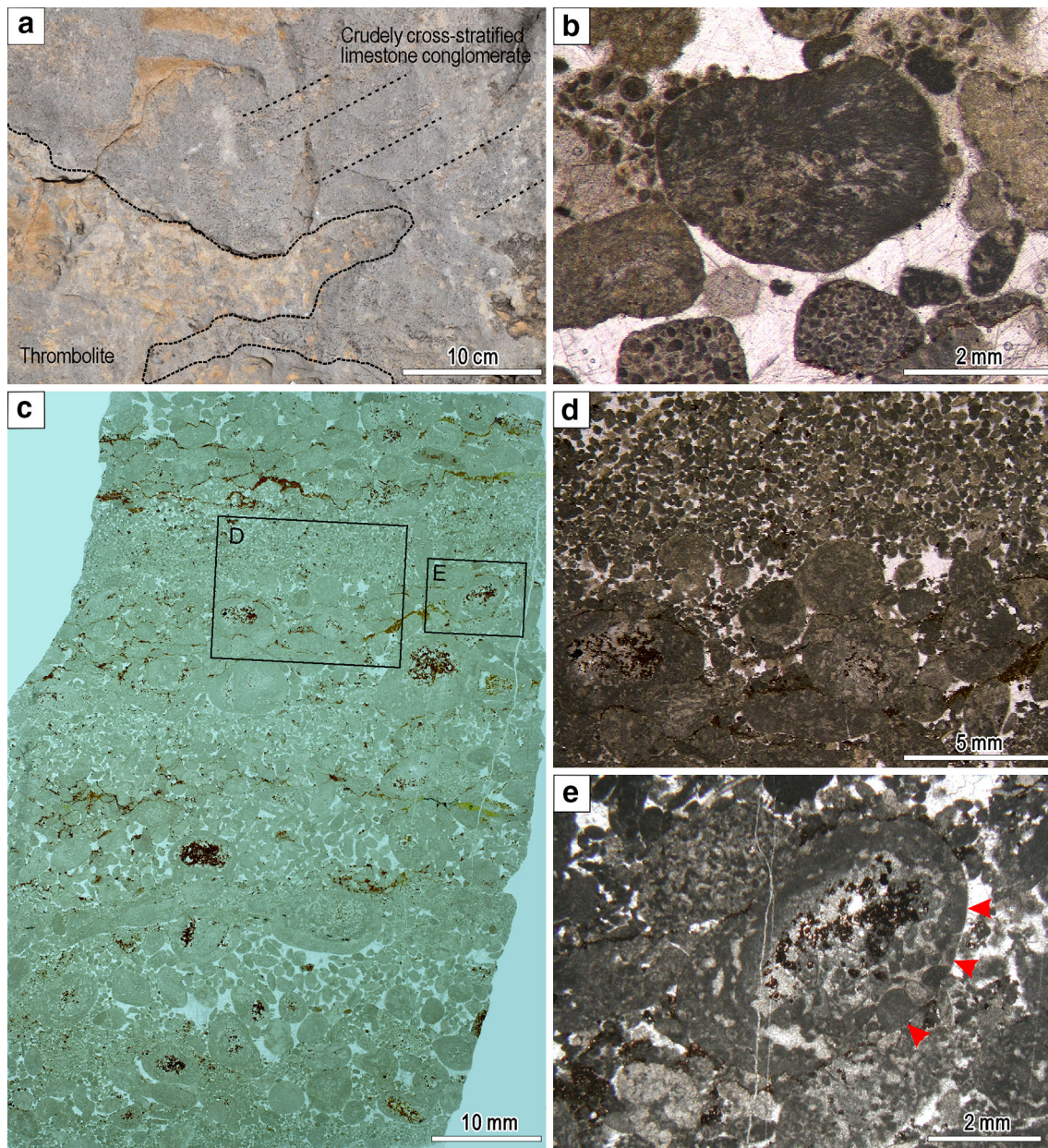
Fig. 9 Microbialite intraclasts. a Crudely cross-stratified limestone conglomerate and associated thrombolite bioherm with an irregular erosion boundary. The clasts of conglomerate are mostly oval and rounded; the size ranges from a few mm to a few cm, resembling full-cortex oncoids. b Photomicrograph of intraclasts that are composed of either calcified microbes ( center ) or peloids. Note the sharp edges of
