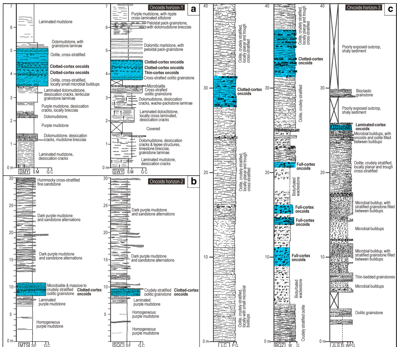
Fig. 3 Detailed columnar sections showing occurrences of the oncoids in the Shandong region. a Lower part of the Mantou Formation in SMY and SWY sections. b Upper part of the Mantou Formation in MTS and SQC sections. c Lower part of the Zhangxia
