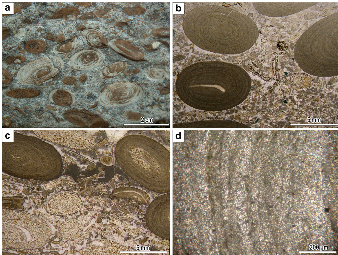
Fig. 6 Laminated-cortex oncoids. a Partly dolomitized (dark-color part) oncoids with a thick, well-laminated cortex. b Smooth-outlined and concentric oncoids with well-laminated cortices and nuclei of small bioclasts in a bioclastic grainstone. Note an oncoid does not
