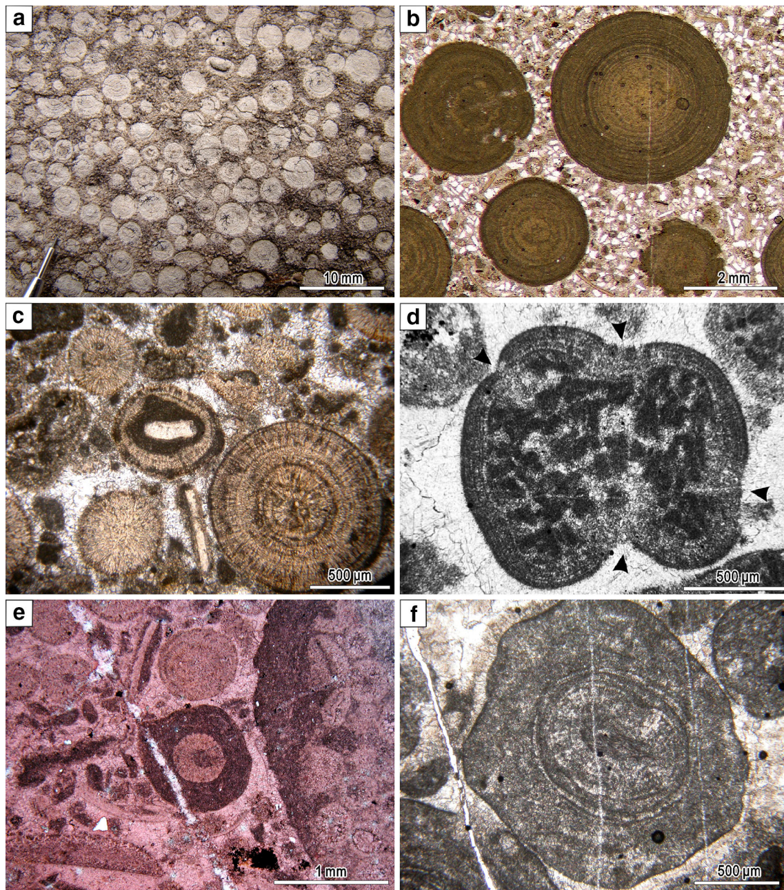
Fig. 10 Microbial ooids. a An outcrop photo showing large ooids (some are broken). b Giant ooids with concentric micritic cortex in the matrix of quartz grains and bioclasts. c An ooid ( center ) with a micro-oncoid as nucleus. d An ooid with a fragment of Epiphyton colonies as nucleus (from Woo et al. 2008). Arrow heads indicate
