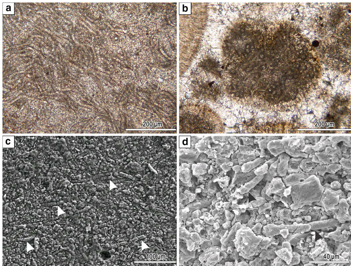
Fig. 4 Photomicrographs of calcified cyanobacteria, Girvanella . a Tubular filaments of Girvanella . b Transverse section of tubular Girvanella , showing circular feature. c SEM photo showing thread-
