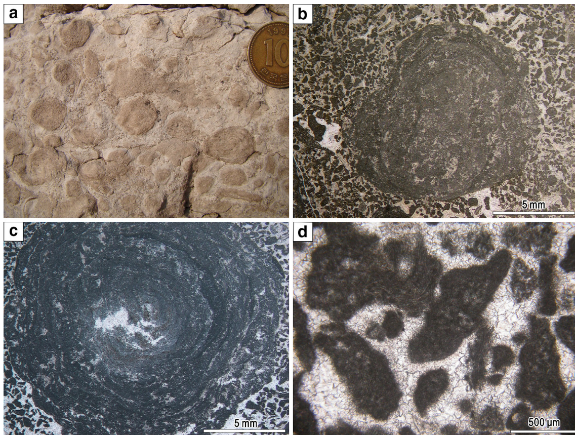
Fig. 8 Full-cortex oncoids. a Outcrop photo of spherical nucleus-less, full-cortex oncoids. Coin for scale is 23 mm in diameter. b An irregular-shaped oncooid with crudely laminated (clotted) texture in a
