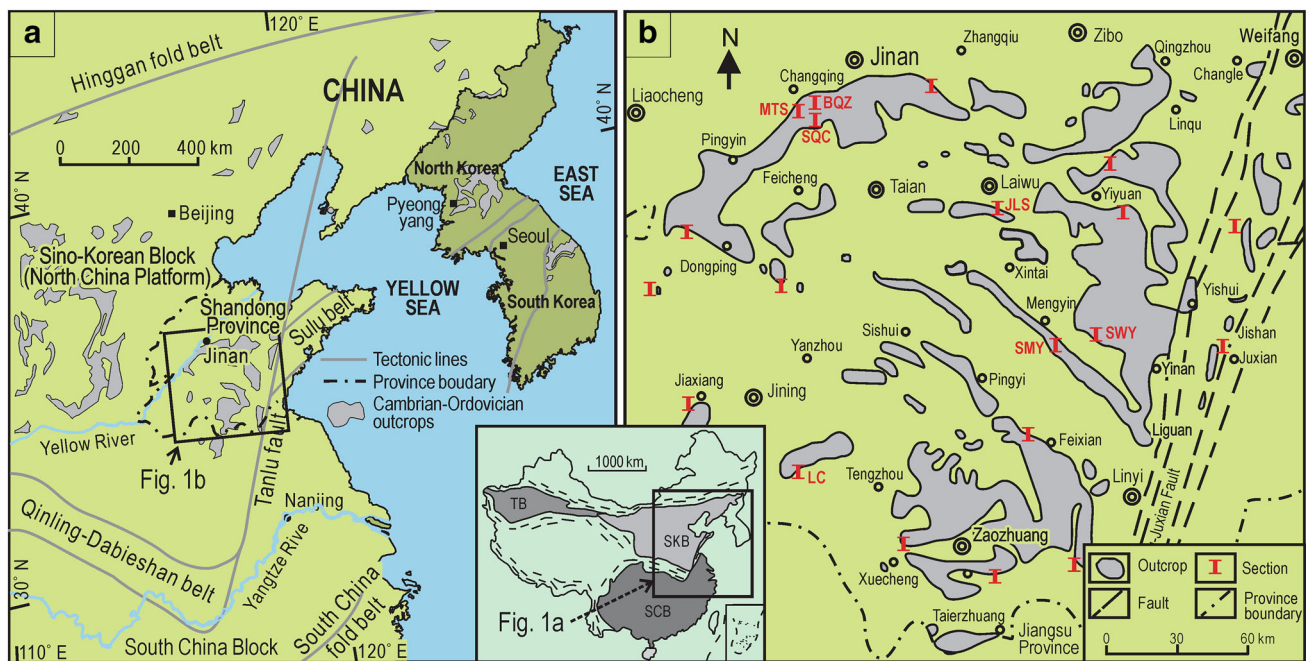
Fig. 1 a Major tectonic boundaries and Cambrian–Ordovician outcrops of the North China Platform. b Outcrop sections that yield oncoids from the Mantou and Zhangxia formations (Cambrian Series 2–3) in Shandong Province, China. MTS Mantoushan section, SQC
