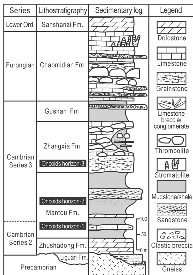
Fig. 2 Schematic stratigraphic succession of the Cambrian in Shandong Province, China. The oncoids occur only in the Mantou and Zhangxia formations
