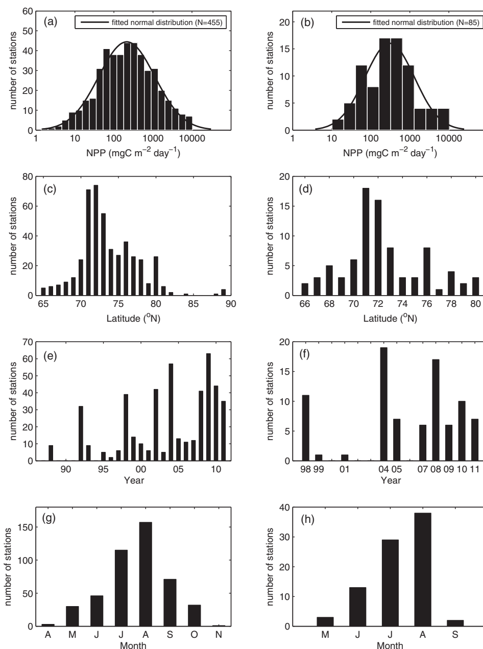
Figure 2. (left) In situ integrated NPP at the N=455 in situ sampling stations and (right) from the N=85 satellite match-up stations shown in Figure 1. Figures 2a and 2b are the distribution of in situ integrated NPP. Figures 2c and 2d, Figures 2e and 2f, and Figures 2g and 2h show where and when those in situ NPP were measured in terms of latitude, year, and month, respectively.
