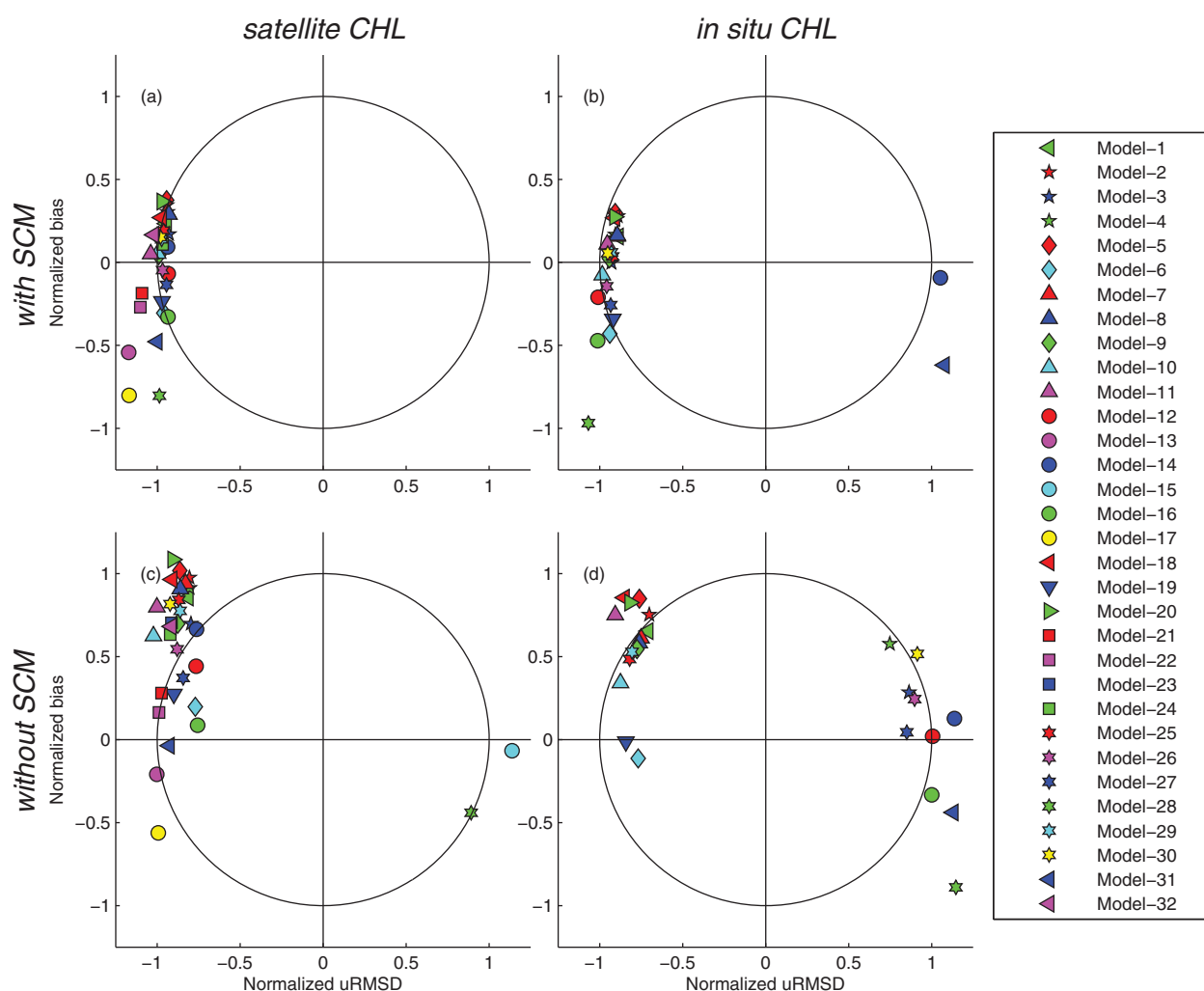
Figure 10. Target diagrams of (a) Case 1 using satellite chlorophyll (CHL) and (b) Case 9 using in situ CHL based on the stations where SCM existed (N=44), and (c) Case 1 and (d) Case 9 based on the stations where SCM was not present (N=39) among the 85 stations (1998–2011) in Figure 5. Note that two stations were excluded because no SCM information was available.
