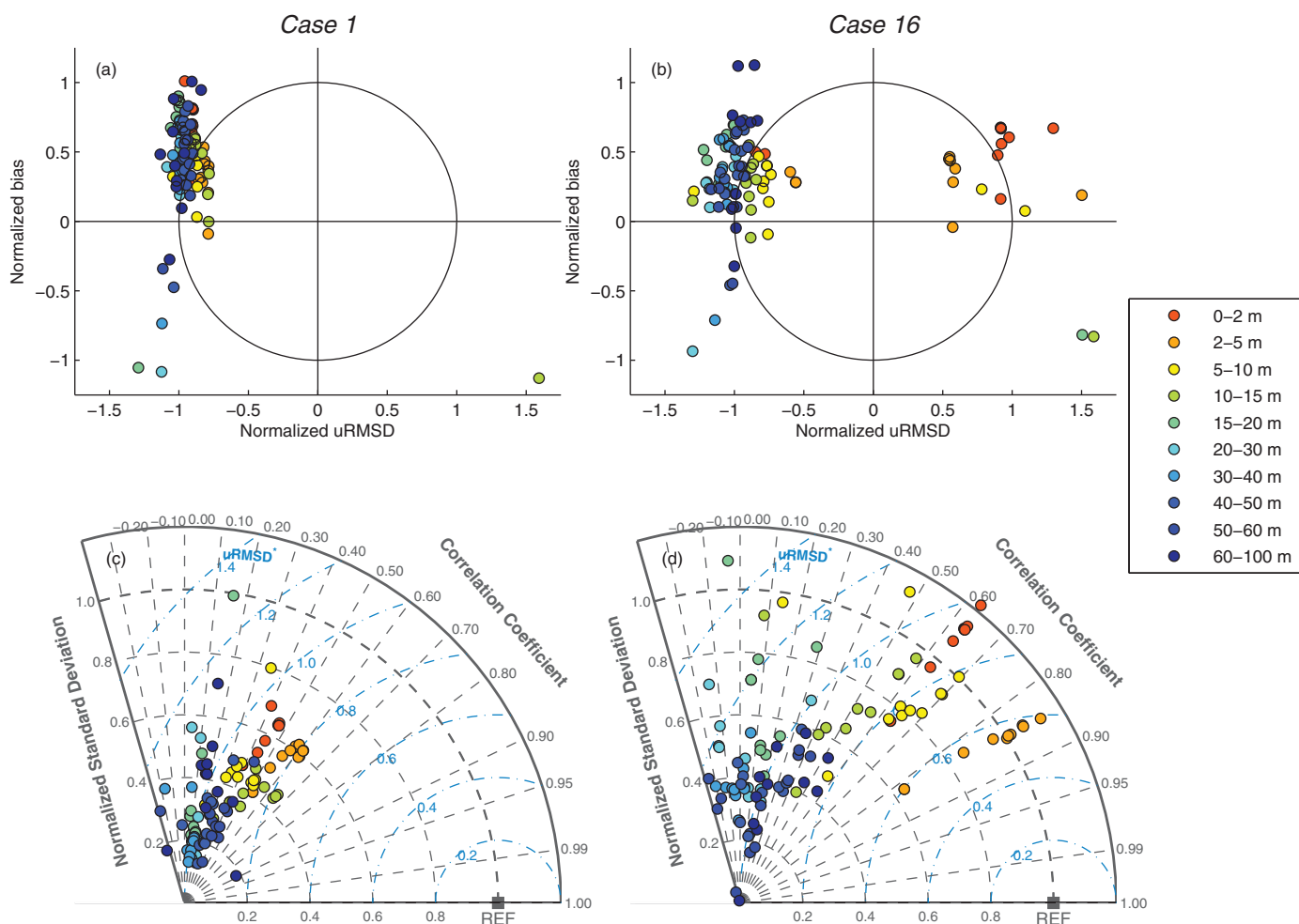
Figure 13. (a, b) Target and (c, d) Taylor diagrams of (left) Case 1 and (right) Case 16, representing relative model performance in reproducing \log\text{NPP}_{N=85} by the 11 depth-resolved models (Models 1–8, 12, 14 and 16) using satellite and in situ chlorophyll, respectively. The symbols indicate the statistics between in situ and estimated NPP at various depth layers: 0–2 m, 2–5 m, 5–10 m, 10–15 m, 15–20 m, 20–30 m, 30–40 m, 40–50 m, 50–60 m, and 60–100 m.
