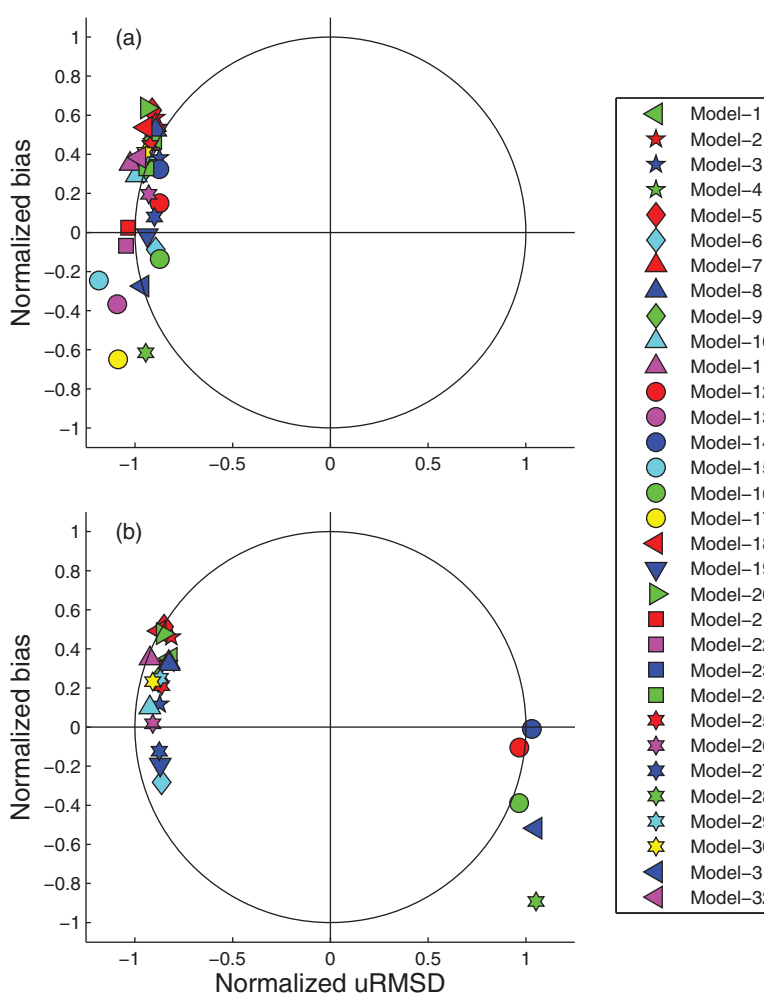
Figure 6. Target diagrams illustrating relative model performance in reproducing \log NPP_{N=85} using (a) satellite chlorophyll (Case 1) and (b) in situ chlorophyll (Case 9).
