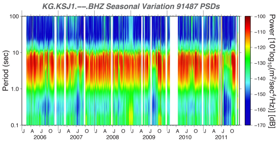
Figure 3. Spectral amplitude variation in seismic noise for BHZ (broadband vertical component) during the period of 2006-2011. Note that the seismic energy at the frequency range of DF microseisms (4-8 s) becomes weaker during July to September annually, which is a different behavior from that of the northern hemisphere except the Arctic region. Empty spaces in the plot indicate data missing or a period of malfunctioning.
