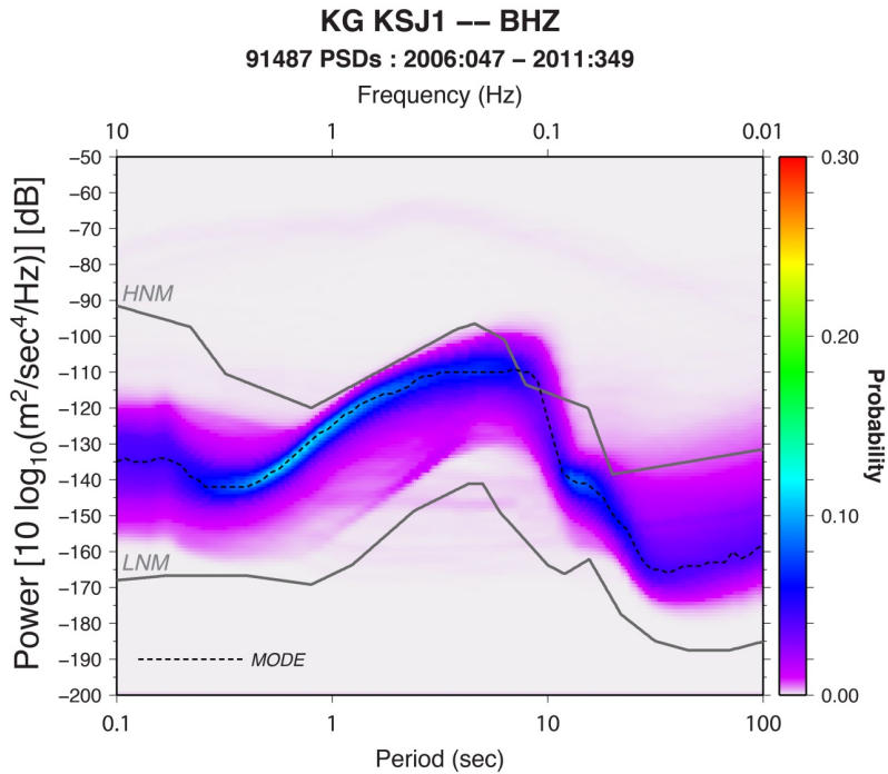
Figure 2. A Probability Density Function (PDF) plot of BHZ for KSJ1 during 2006-2011. Two predominant peaks appear around 5 and 10 s in period, corresponding to secondary (or DF) and primary microseisms, respectively. HNM and LNM indicate the standard high and low noise model (Peterson, 1993), respectively. The most probable energy with respect to frequency is presented by a dashed curve (mode).
